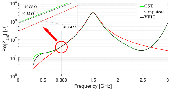
Fig. 5. Resistance of the designed antenna (CST), of the VFIT model and of the model extracted by the graphical method.
