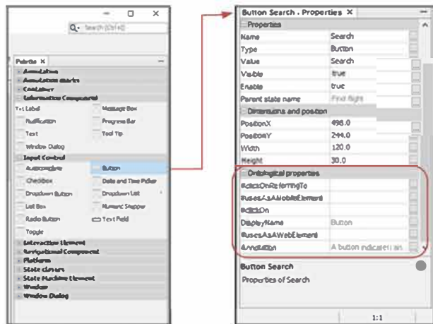
Figure 13 Pallets with the widget Button and its properties extracted from the ontology
