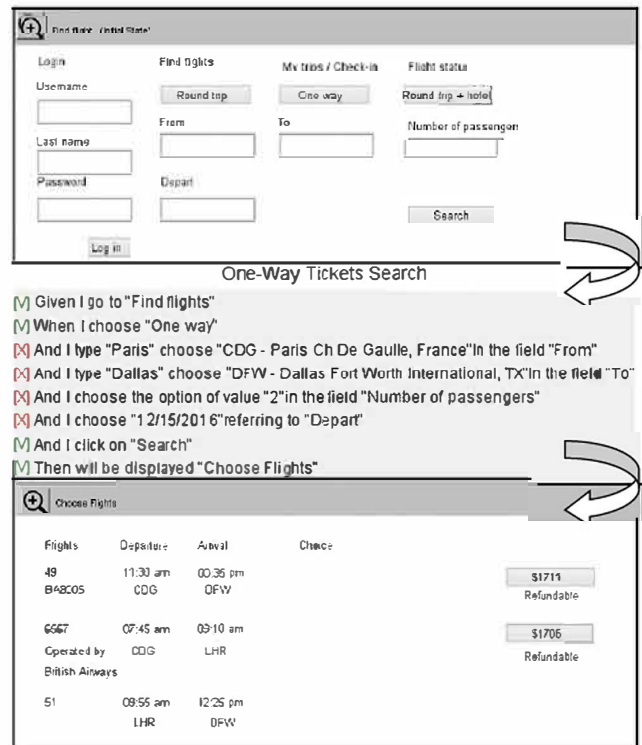
Figure 14 A State Machine Transition between sketches of a PANDA Prototype for the User Story "Flight Tickets Search" From top to bottom: the initial State "Find Flights", a Transition represented by the Scenario "One-Way Tickets Search", and finally the resultant State "Choose Flights"
