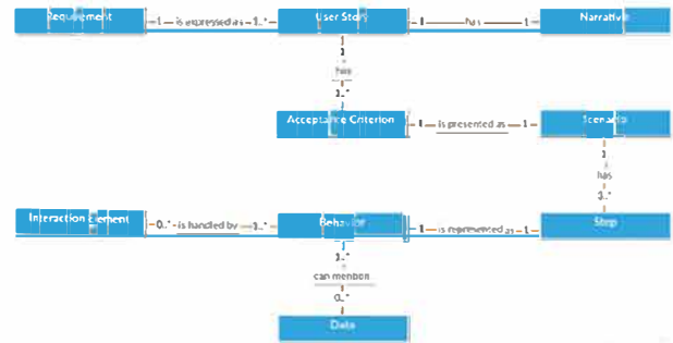
Figure 2 Conceptual Model of User Requirements
