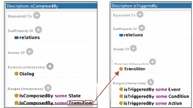
Figure 8 Object Properties isComposedBy (left) and isTriggeredBy (right)
