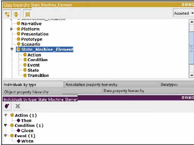
Figure 6 State Machine Elements and their Individuals
