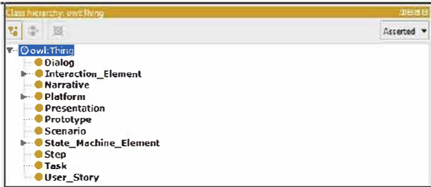
Figure 3 Root classes of the ontology
