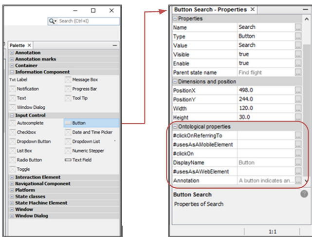
Figure 13. Palettes with the widget Button and its properties extracted from the ontology.
