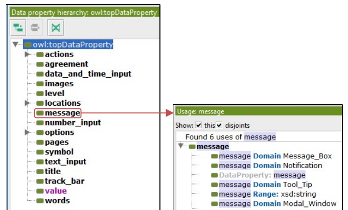
Figure 5. (a) Left: Data Properties. (b) Right: Data Property “message”
