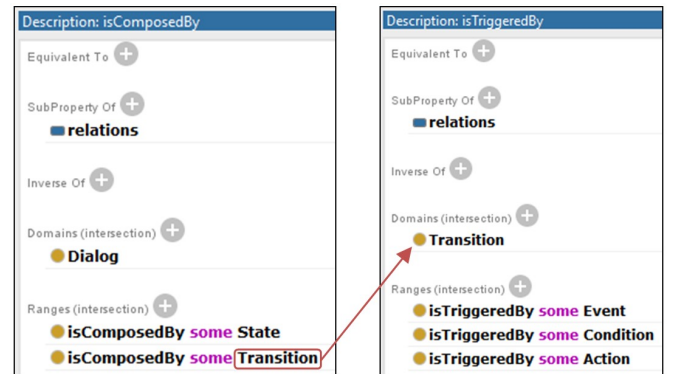
Figure 8. Object Properties isComposedBy (left) and isTriggeredBy (right)
