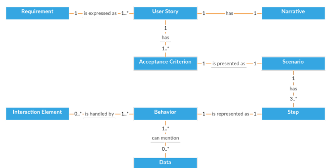
Figure 2. Conceptual Model of User Requirements
