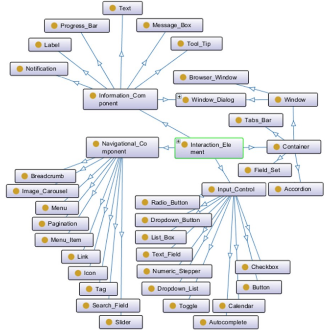
Figure 4. Cloud of User Interface Elements
