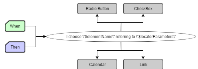
Figure 9. Components on the ontology used to specify a behavior
