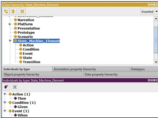
Figure 6. State Machine Elements and their Individuals
