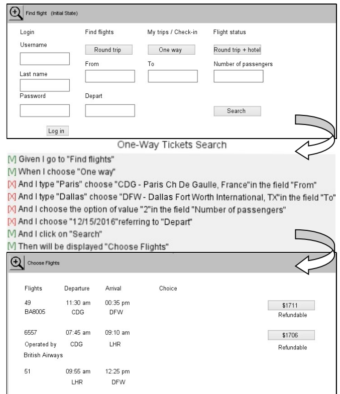
Figure 14. A State Machine Transition between sketches of a PANDA Prototype for the User Story "Flight Tickets Search". From top to bottom: the initial State "Find Flights", a Transition represented by the Scenario "One-Way Tickets Search", and finally the resultant State "Choose Flights".
