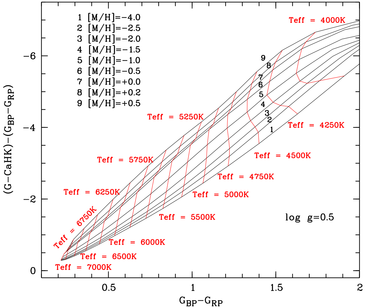
Figure 11. The theoretical colour-colour plane (G_{BP} - G_{RP}) , [(G - \text{CaHK}) - (G_{BP} - G_{RP})] for a fixed surface gravity \log g = 0.5 . Lines of constant metallicity are shown in black and those of constant T_{\text{eff}} in red.
