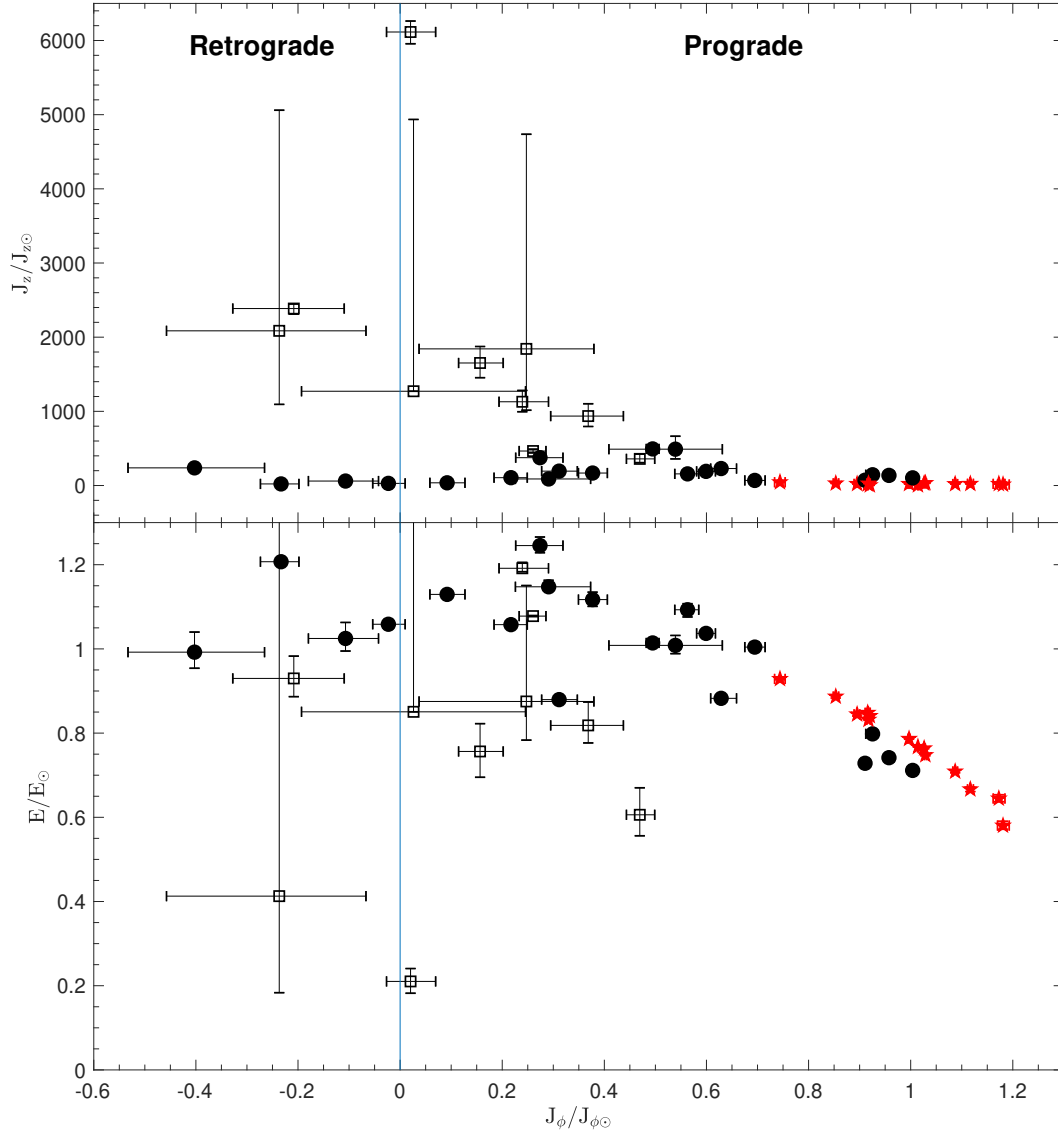
Figure A2. The specific energy versus rotational action J_{\phi} (also known as specific angular momentum L_z ) diagram for our stars (lower panel) and the J_z action (as defined in equation 6 of Binney 2012 ) versus rotational action (upper panel). All the quantities are normalized to the solar value. The symbols are the same as in Fig. A1.
