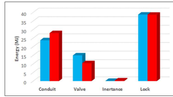
Fig. 3. Energy in the system for the default model (blue) and modified valve law model (red)
