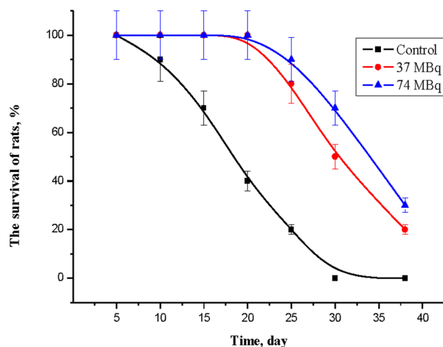
Figure 4. Assessment of therapeutic effect. Survival curves for Wistar rats with implanted cholangioma RS-1 after intratumoral injection of the Si*NPs-PEG- ^{188}\text{Re} conjugates providing different doses of radioactivity (37 and 74 MBq) and for control group injected with physiological solutions. Each group was composed of 10 animals.
