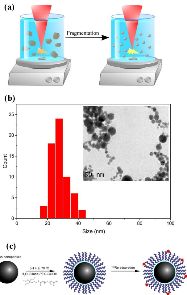
Figure 1. Synthesis and functionalization of Si nanoparticles for nuclear medicine tasks. (a) Schematic of laser synthesis of Si* NPs. Crystalline Si microcolloids ( \sim 0.5 \mu\text{m} in size), preliminarily prepared by mechanical milling of a Si wafer, are dispersed in deionized water and illuminated by focused radiation from fs laser. The laser-ablative process leads to the formation of spherical, small size-dispersed Si* NPs exempt of any toxic impurity; (b) Typical transmission electron microscopy image (inset) and corresponding size distribution of Si* NPs prepared by fs laser ablation; (c) Schematic presentation of functionalization protocol for the coating of Si* NPs by polyethylene glycol (PEG) and subsequent decoration by radioactive ^{188}\text{Re} atoms. All images were designed and drawn by authors of this manuscript.
