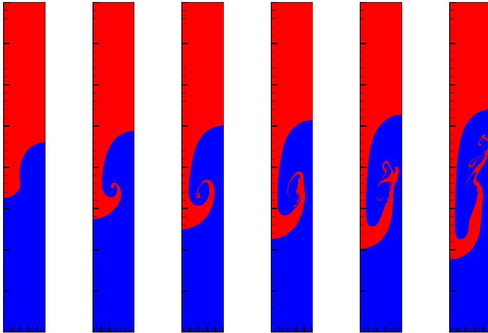
FIGURE 3. \mathfrak{Re} = 3000 ; \mathfrak{Bi} = 0 , \alpha_1 = \alpha_2 = 0 ; density ratio 3. The interface is shown at times 1, 1.5, 1.75, 2, 2.25 and 2.5. The heavier fluid (\rho_2, \mu_2, \alpha_2) corresponds to the red zone.
