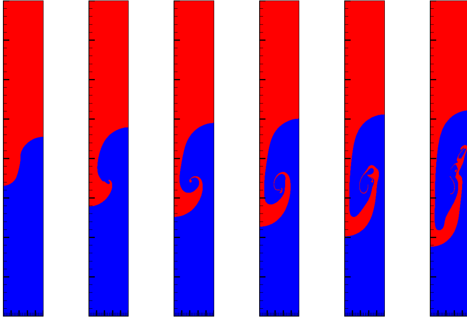
FIGURE 4. \mathfrak{Re} = 3000 ; \mathfrak{Bi} = 10 , \alpha_1 = 0 , \alpha_2 = 1 ; density ratio 3. The interface is shown at times 1, 1.5, 1.75, 2, 2.25 and 2.5. The heavier viscoplatic fluid ( \rho_2, \mu_2, \alpha_2 ) corresponds to the red zone.
