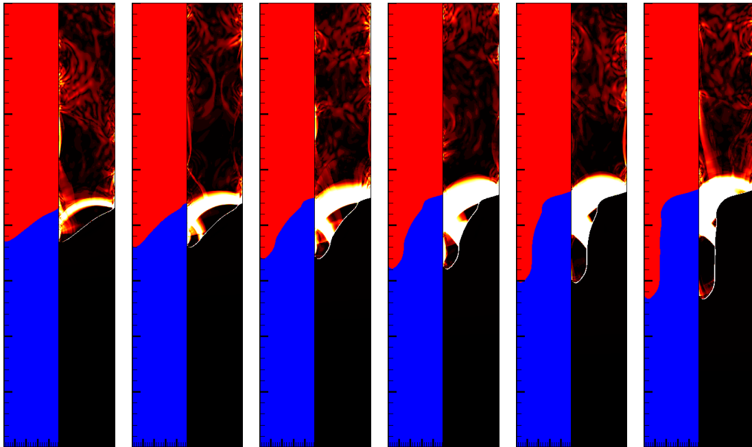
FIGURE 5. \mathfrak{Re} = 3000 ; \mathfrak{Bi} = 100 , \alpha_1 = 0 , \alpha_2 = 1 ; density ratio 3. Interface (left) and deformation rate \|\mathbf{D}\mathbf{u}\| in the viscoplastic phase (right) are shown at times 1.5, 2, 2.5, 2.75, 3 and 3.25. The heavier fluid ( \rho_2, \mu_2, \alpha_2 ) corresponds to the red zone.
