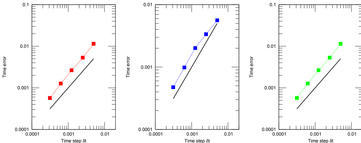
FIGURE 2. Error for the velocity, pressure and density in L^2(\Omega) -norm. The slope of the solid black line is 1 corresponding to an error in O(\delta t) .
