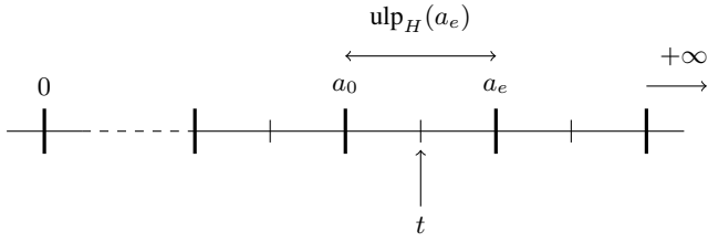
Fig. 2: Halfway case 1: t = a_e - (1/2)\text{ulp}_H(a_e) , where t = a_e + b_e . We have a_0 = a_e - \text{ulp}_H(a_e) and b_0 = -b_e .
