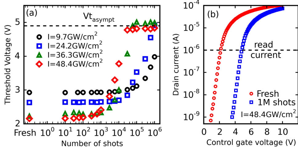
Figure 3. (a) Evolution of experimental V_t of erased cells as a function of the number of laser shots at different intensities ( V_{CG} = 0 V). (b) Evolution of the drain current as a function of the control gate voltage before and after 1 million laser shots at 48.4 GW/cm 2 .
