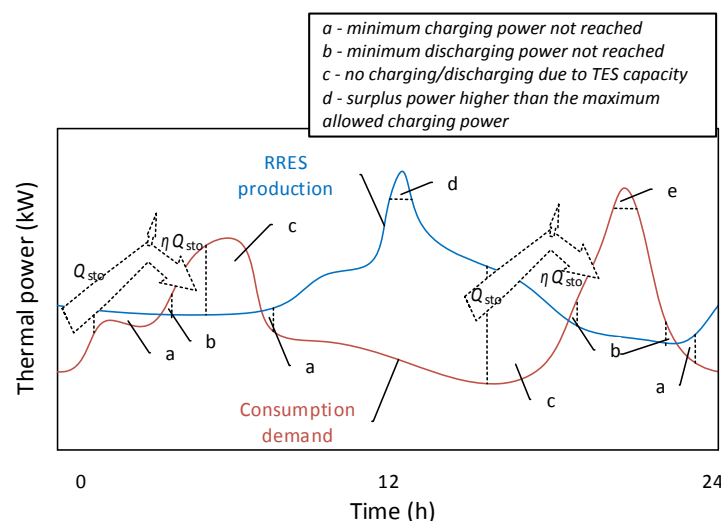
Figure 1. Estimation of waste energy recovery potentials with a simplified TES model.
