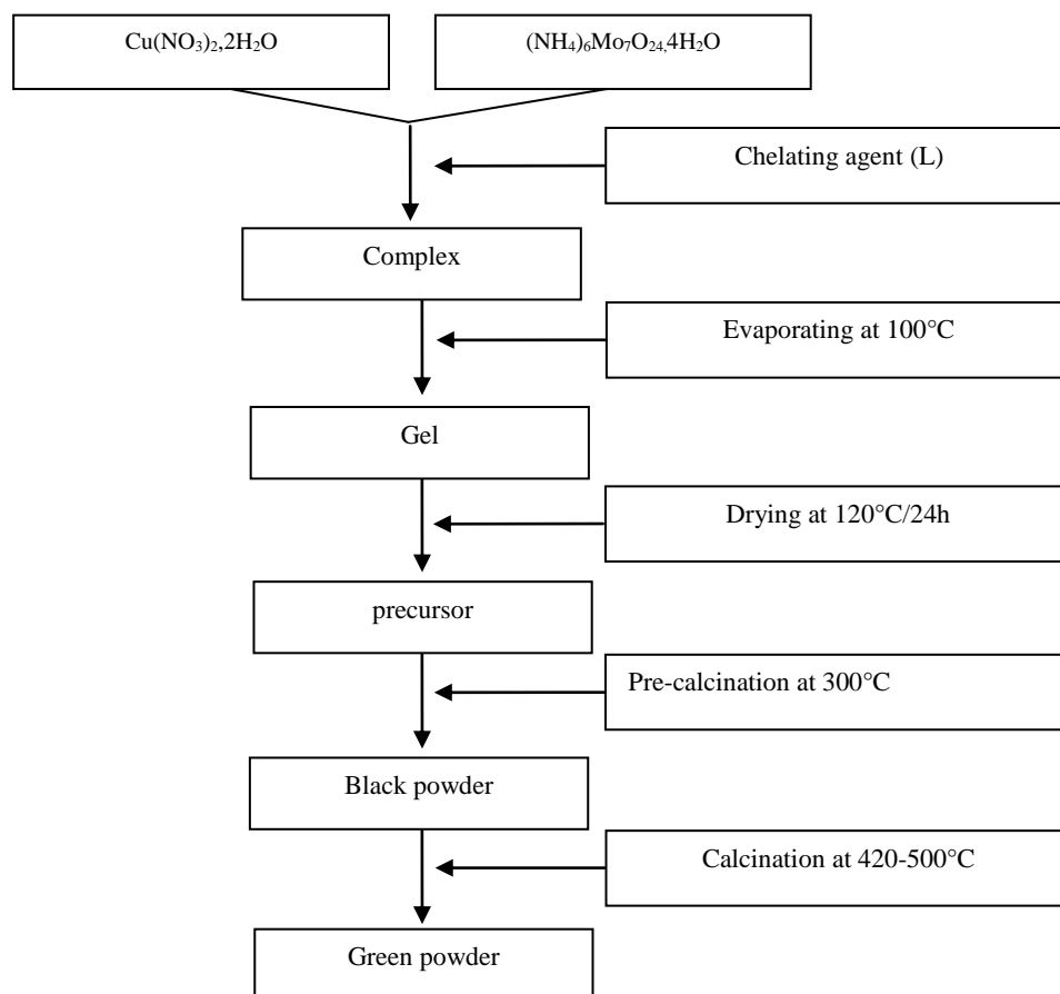
Figure1: Flowchart of the synthesis of \text{CuMoO}_4 powder
