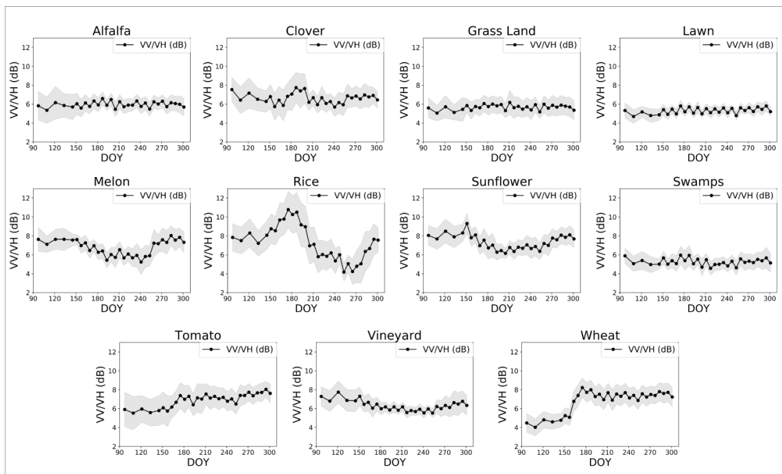
Figure 5. Temporal evolution of the ratio VV/VH for SAR backscattering coefficient \sigma^0 of 11 crop types. Mean values are represented by dots and standard deviations are represented by the filled color domains surrounding the curves.
