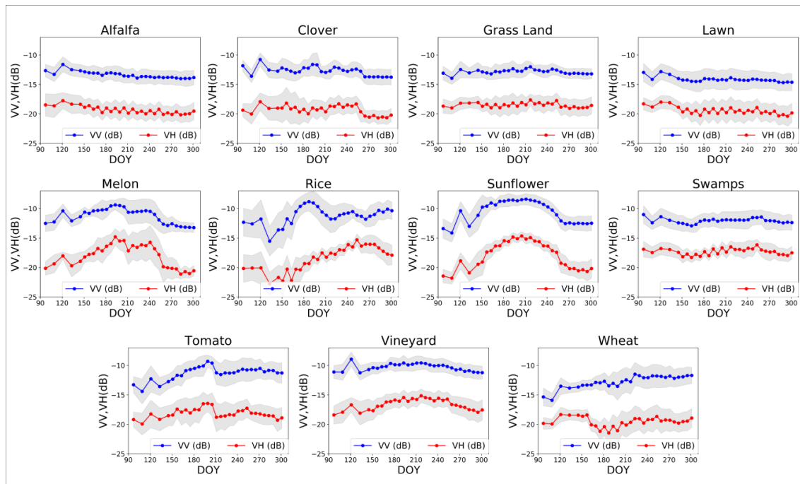
Figure 4. Temporal evolution of SAR backscattering coefficient \sigma^0 of 11 crop types for VV and VH polarizations. Mean values are represented by dots and standard deviations are represented by the filled color domains surrounding the curves.
