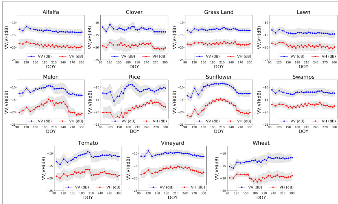
Figure 4. Temporal evolution of SAR backscattering coefficient \sigma^{\circ} of 11 crop types for VV and VH polarizations. Mean values are represented by dots and standard deviations are represented by the filled color domains surrounding the curves.
