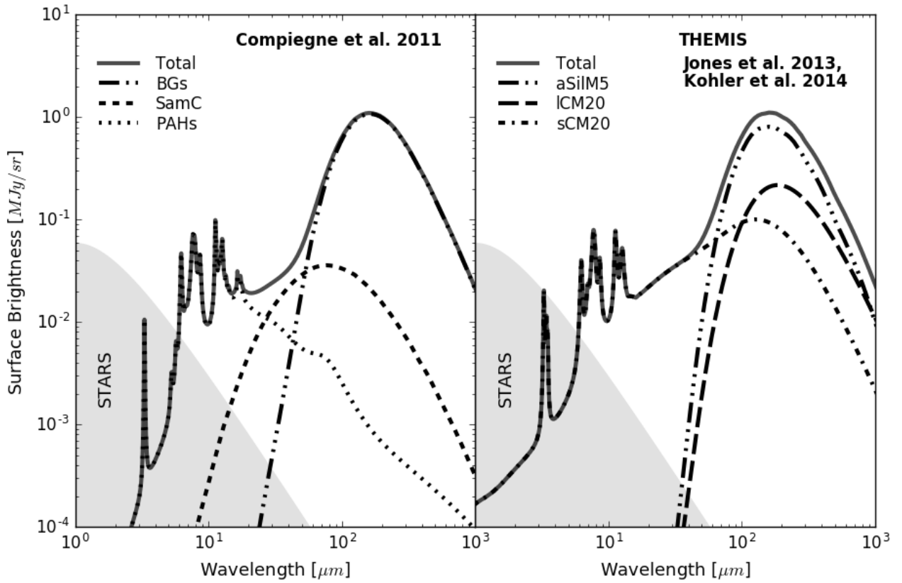
Fig. 1. Original Compiegne et al. (2011; MC11 model, left) and THEMIS ( right ), for U = 1 (from Mathis et al. 1983 ) and N_{\text{H}} = 10^{20} \text{ H cm}^{-2} . They vary by the total number of components and optical and heating properties. The “stars” component is scaled with a blackbody at 5000 K.
