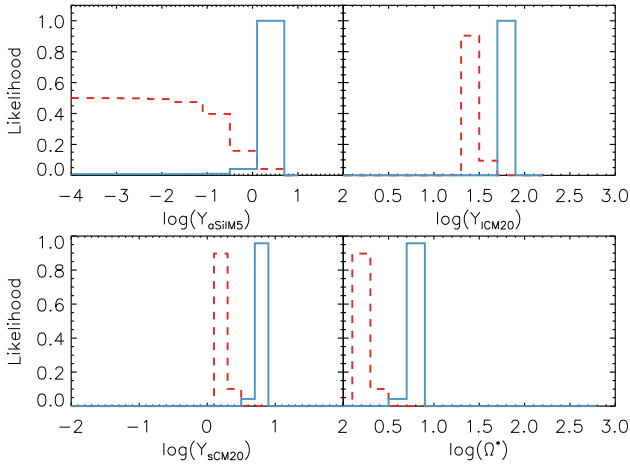
Fig. 7. Marginalized and normalized likelihoods of the Y_{\text{aSiIM5}} , Y_{\text{ICM20}} , Y_{\text{sCM20}} , and \Omega^* parameters for two pixels in the SMC: a pixel showing an upper-limit in the Y_{\text{aSiIM5}} fit (red-dashed line) and a pixel showing well-constrained fits (blue line).
