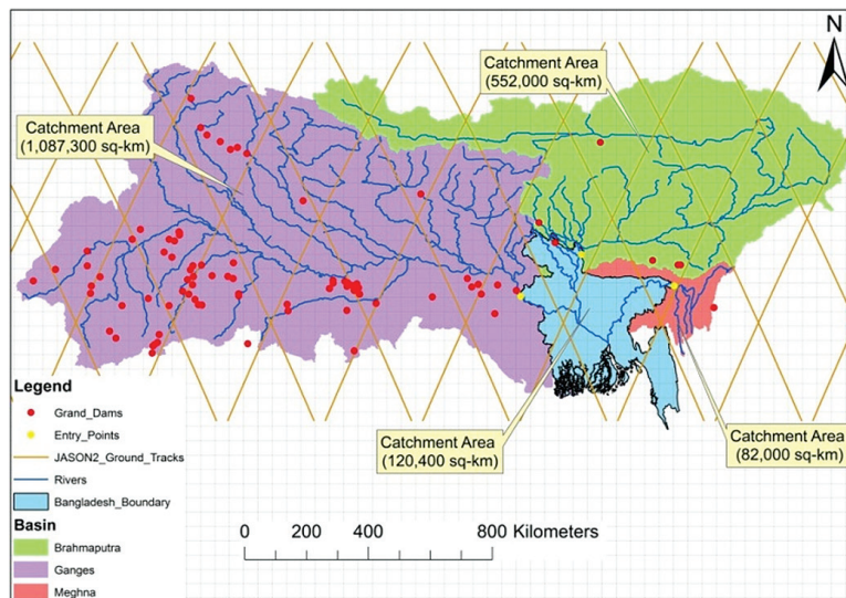
FIG. 1. Map of Ganges–Brahmaputra basin showing Bangladesh’s location as the smallest, most downstream, and most flood-prone country in the basin. The locations in red are dams; cross tracks in brown represent Jason-2 satellite paths.
