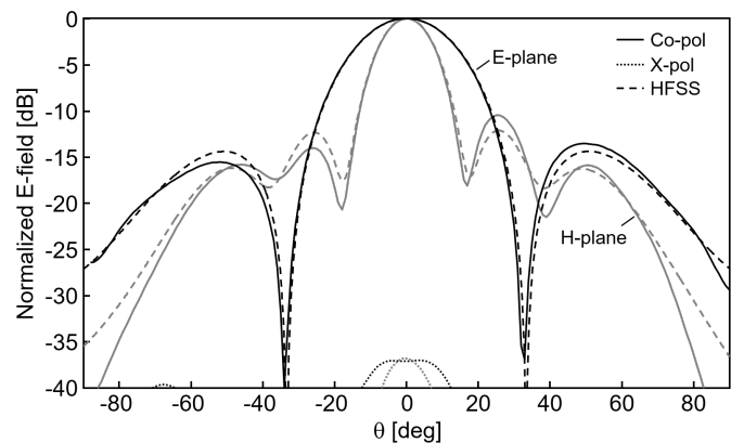
Fig. 5. Normalized radiation patterns of the array for a uniform illumination along the E and H-plane for broadside radiation at 5.8 GHz.
