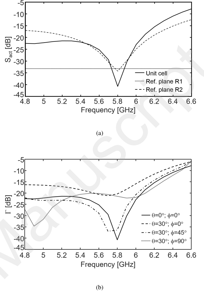
Fig. 2. Active reflection coefficient of a unit cell of the array in an infinite periodic environment. (a) At the reference planes R1 and R2 in Fig. 1 for broadside radiation. (b) At the SMA connection for different scanning angles and planes of observation.
