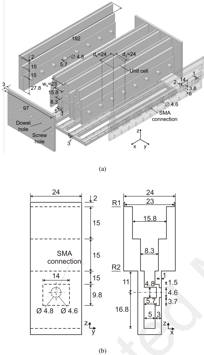
Fig. 1. The 8 \times 4 CTS array. (a) Perspective view. The unit cell of the array is outlined by a dashed box. (b) Side view of the unit cell of the array along the yz - and xz -planes. The dimensions are in mm .
