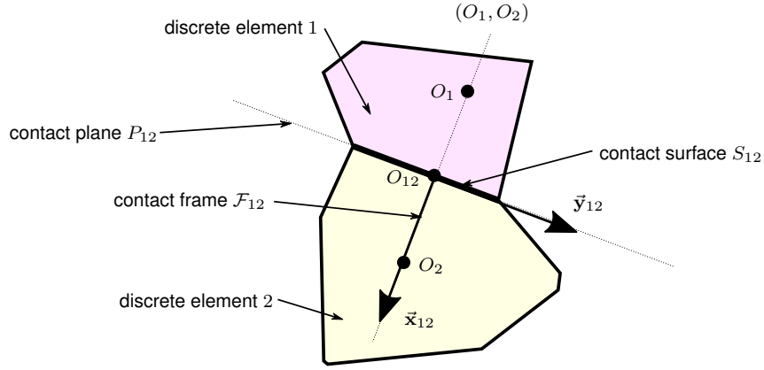
Figure 2: Configuration of the contact problem in 2D
