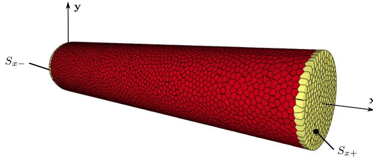
Figure 11: Cylindrical sample
