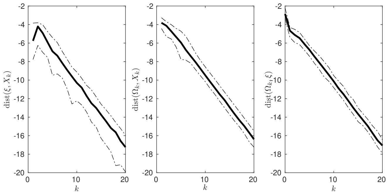
Figure 3: Logarithmic plot of \text{dist}(\xi, X_k) , \text{dist}(\Omega_k, X_k) and \text{dist}(\Omega_k, \xi) . Shown is the median value (oblique line) along with confidence intervals (dashed) covering all but the top and lower 5%.
