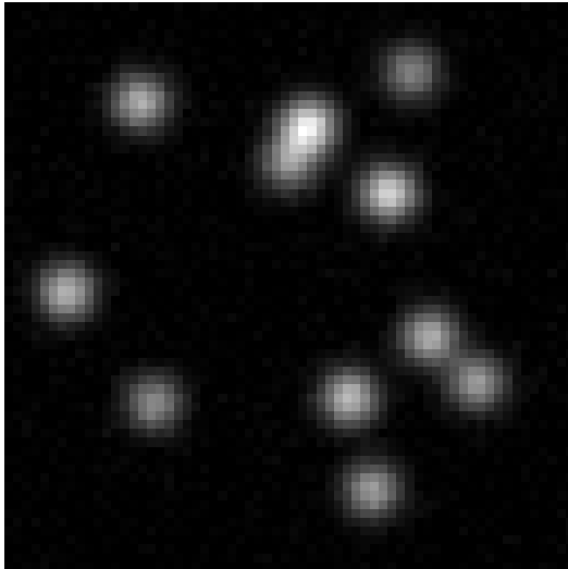
Figure 5: Measurements y associated to a super-resolution experiment. A sparse measure is convolved with a Gaussian kernel and Gaussian white noise is added.
