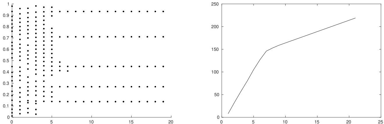
Figure 2: Left: The set X_k of added points for each iteration along a run of the algorithm. Right: The total number of points in \Omega_k along the same run.
