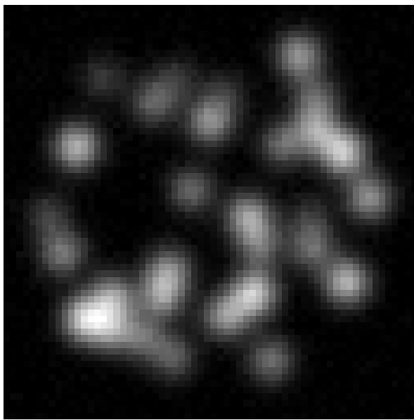
(a) Measurements y (dense)
