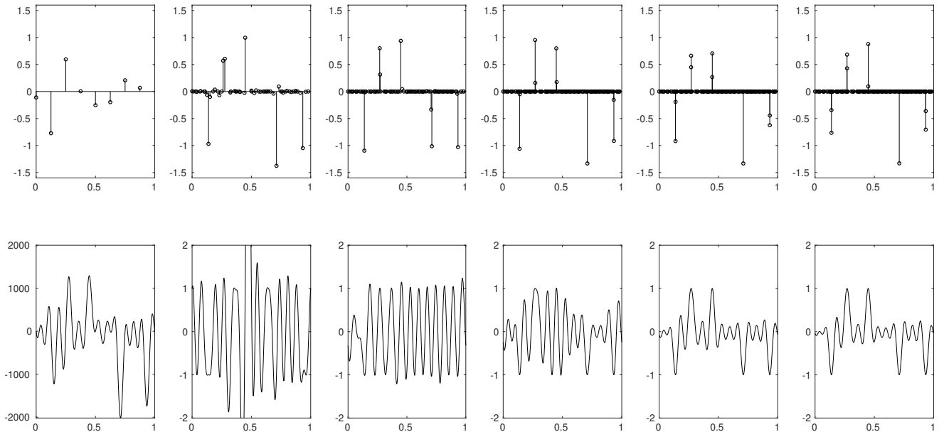
Figure 1: Above: \mu_k for k = 0, 2, 4, 6, 8, 20 along one run of the algorithm. Below: A^*q_k for k = 0, 2, 4, 6, 8, 20 along the same run. Note that the range of the first plot is different from the others.
