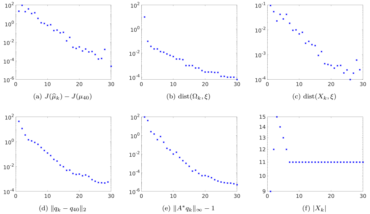
Figure 7: Plot of several quantities of interest along the exchange algorithm's iterates.
