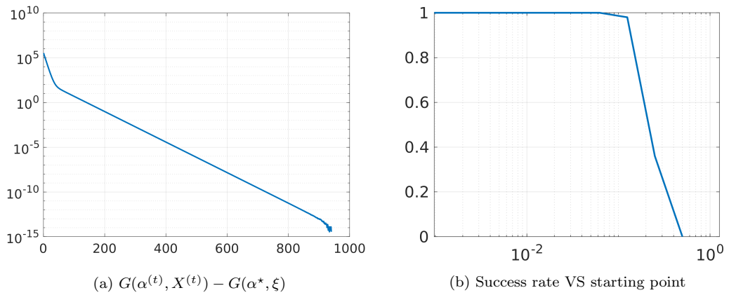
Figure 8: Left: Typical convergence curve in logarithmic scale when the initial guess (\alpha^{(0)}, X^{(0)}) is good enough. Right: Success rate of the continuous descent method over 50 runs of the algorithm, depending on the relative amplitude of the perturbation.
