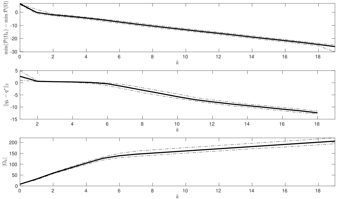
Figure 4: Plot of the evolution optimum gap, q -error and grid sizes. The top two plots are logarithmic, while the bottom one is not. The oblique lines are represent the median iterations, the dashed ones are confidence intervals covering all but the top and bottom 5% values.
