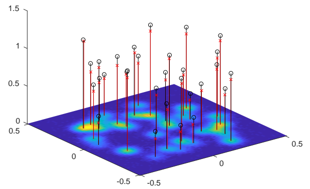
(b) Ground truth and recovered solution
