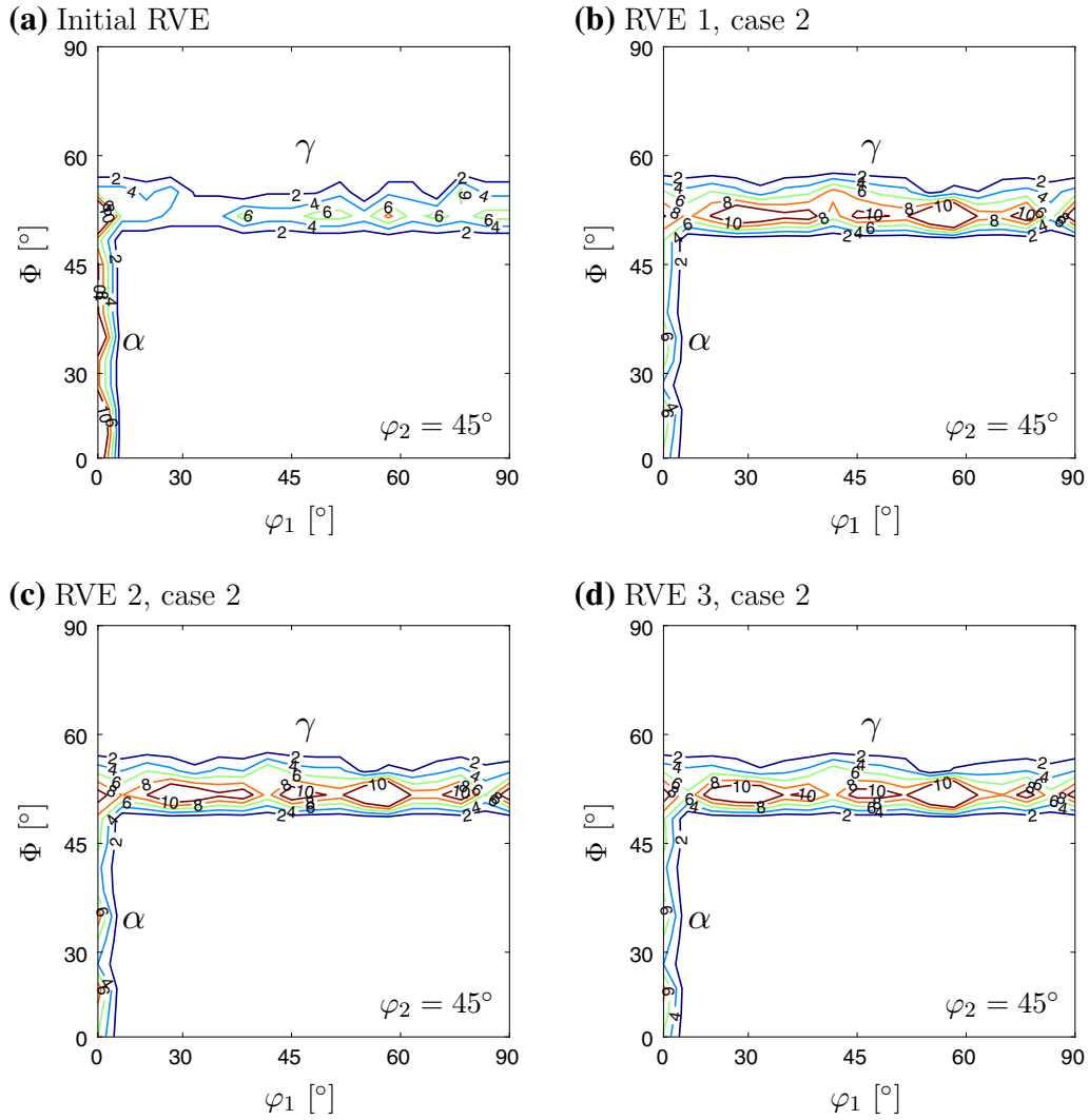
Fig. 10—(a) Initial orientation distribution used in the numerical model, expressed in the Bunge–Euler angles (\varphi_1, \Phi, \varphi_2) . The texture is assumed to consist only of grains belonging to the dominant \alpha - and \gamma -fibers, as shown in Fig. 9. Figures (b) through (d) show the orientation distribution after annealing according to case 2, cf. Table II, for the different RVEs: (b) RVE 1, (c) RVE 2, and (d) RVE 3. In all cases, the \gamma -fiber is strengthened at the expense of the \alpha -fiber after annealing. The same isolines (intensity levels 2, 4, 6, 8, and 10) are plotted in all figures.
