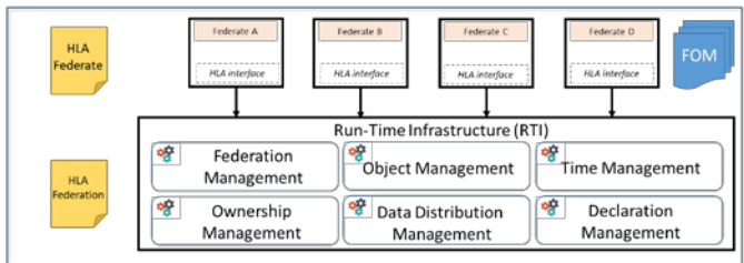
Fig. 1. HLA Architecture diagram.
