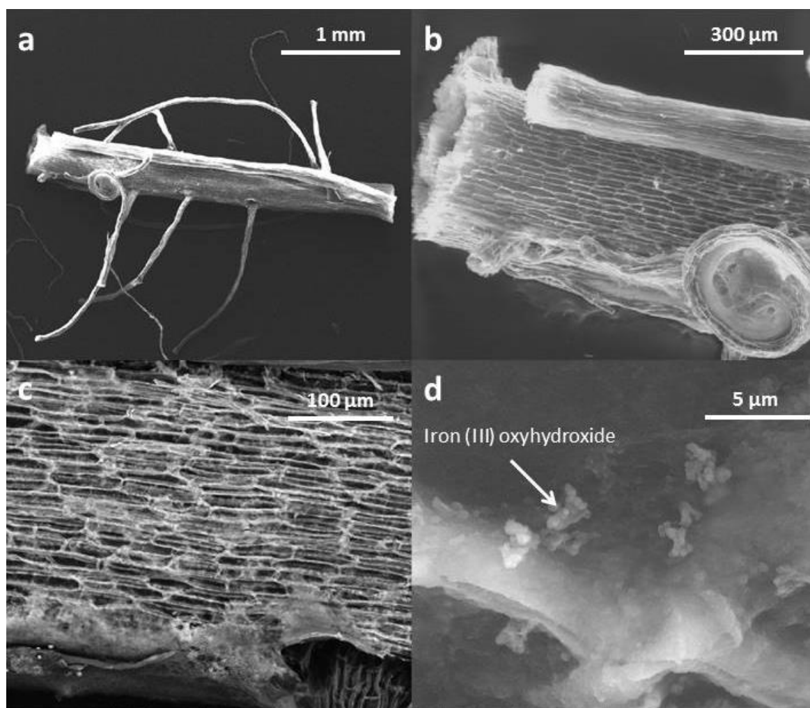
Fig. 4. SEM images of the rice root surface after 14 days of exposure to the 100 \mu\text{mol/L} concentration of Fe (II) sulfate or Fe (II) chloride. (a), (b), (c) and (d) show the iron (III) oxyhydroxide solid phases present on the rice root surface, at increasing resolution.
