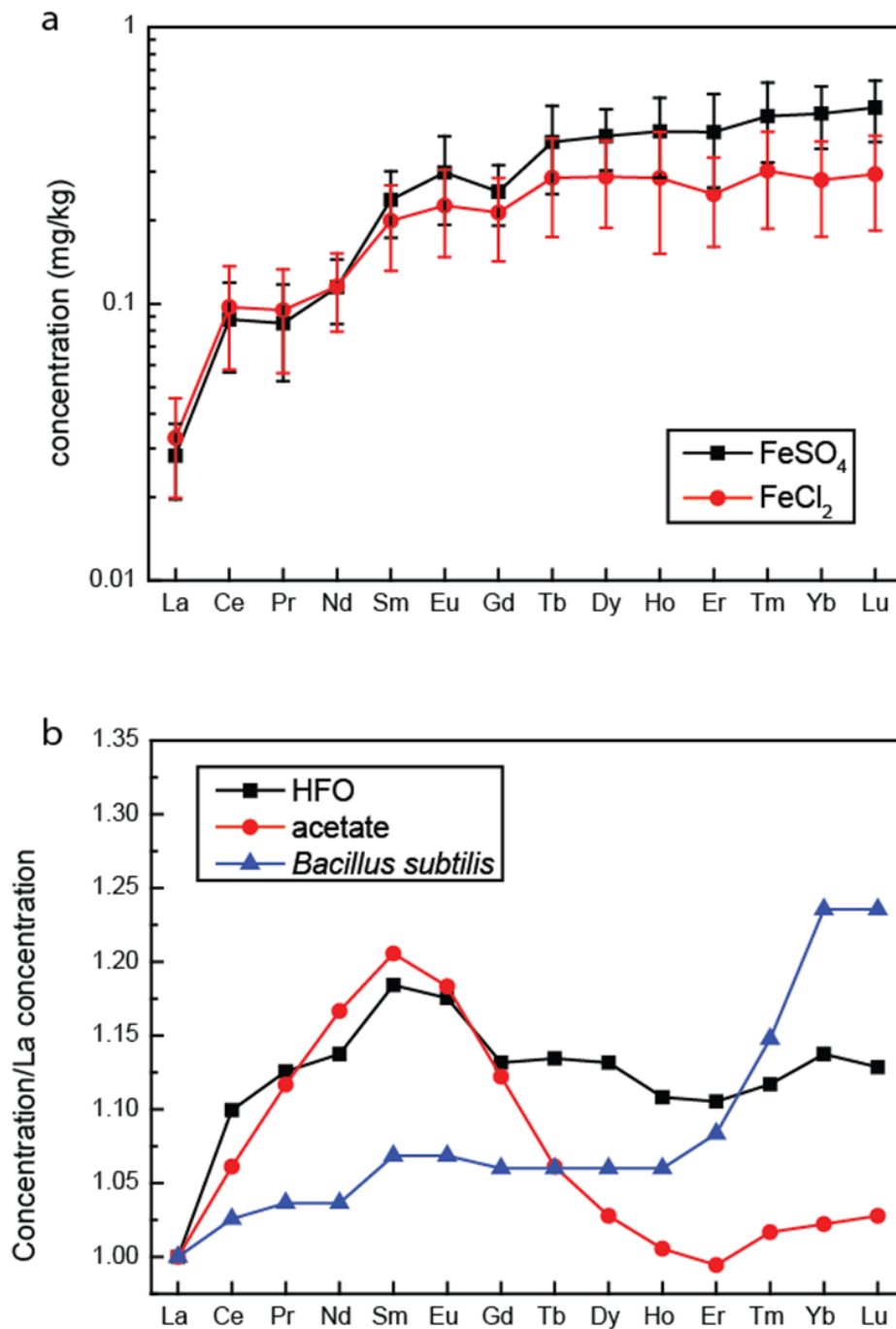
Fig. 7 Rare earth elements patterns of (a) iron plaques (Error bars are shown in the figure, n=2) and (b) HFO, acetate and Bacillus subtilis from literature (Davranche et al., 2004; Byrne and Li, 1995; Martinez et al., 2014). Concentrations are normalized to La for comparison purpose.
