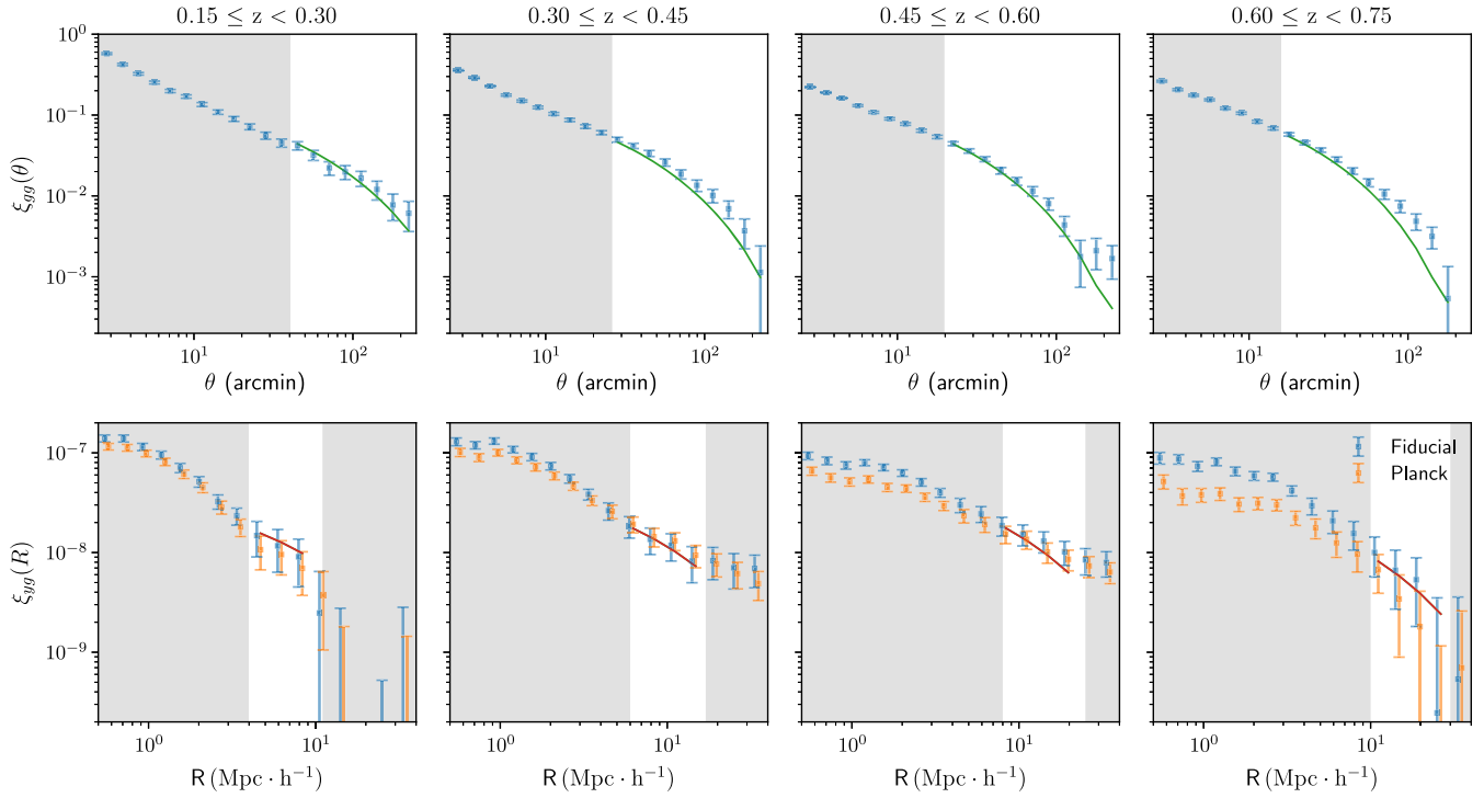
FIG. 6. Measurements of the galaxy autocorrelation (top row) and Compton-y galaxy cross-correlation (bottom row) at different redshift bins corresponding to four redshift bins used in the analysis. The solid line is the best-fit to the fiducial model of Compton-y, which is generated after removing 545 and 857 GHz frequency channels from the analysis. Only data in the unshaded regions are used for fitting. These scale cut choices are validated in Sec. IV E
