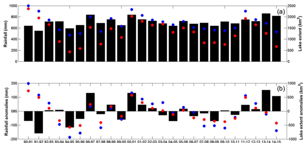
Figure 4. Extent of Poopó Lake (km 2 ) and the variations of the MERGE seasonal amount of rainfall (mm) between 1990 and 2015 (a); and rainfall and lake extent anomalies (b). The maximum and minimum extents are plotted in blue and red, respectively.
