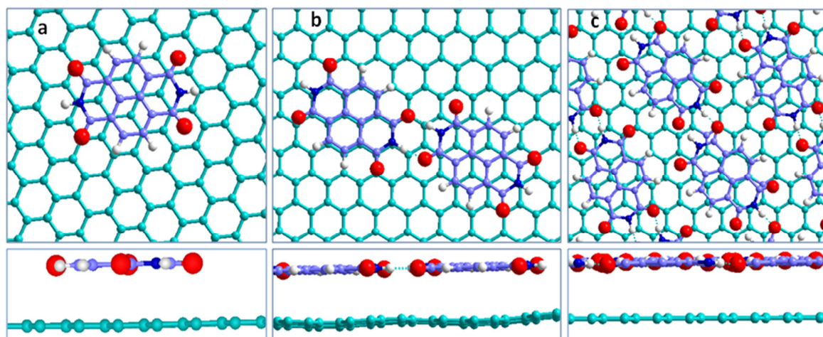
Figure 4: The different most stable structures of NTCDI monomer (a), dimer (b) and 2D-network (c) on graphene surface.
