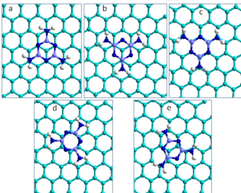
Figure 1: Optimized structures of melamine on different adsorption sites upon graphene: topC-top (a), N-top (b), All-top(c), cross (d), bridge (e). Graphene carbon atoms are in cyan, nitrogen in blue, hydrogen in white, carbon of melamine in lilas.
