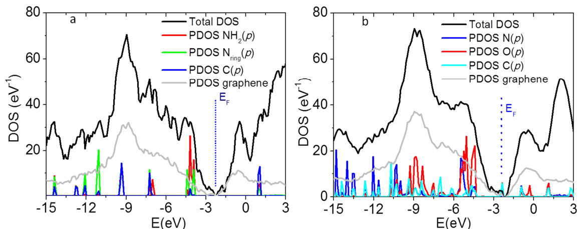
Figure 8: Total DOS (black) of melamine/graphene in the C-top configuration (a) and PDOS on 2p orbitals of Nsp^3 (red), Nsp^2 (green) and C (blue) for melamine. Total DOS of NTCDI/graphene (b) and the PDOS on 2p orbital of N (blue), O (red) and C (cyan) for NTCDI.
