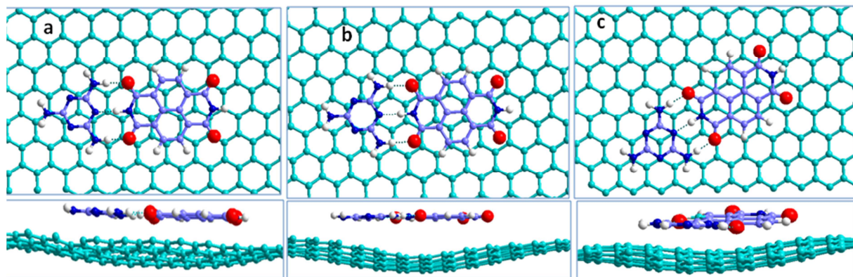
Figure 5. The different optimized structures of Melamine-NTCDI dimer on a graphene sheet. Configurations A (a), B (b), and C (c).
