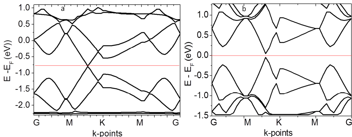
Figure 9. . Band structure of a) pristine graphene and b) graphene under melamine adsorption in C_top configuration.
