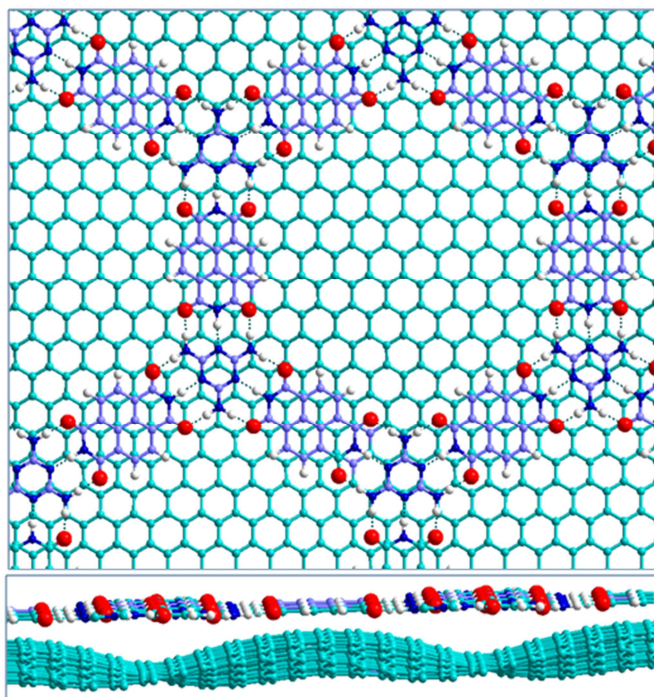
Figure 6. Top view (top) and side view (bottom) of the Melamine-NTCDI 2D network
