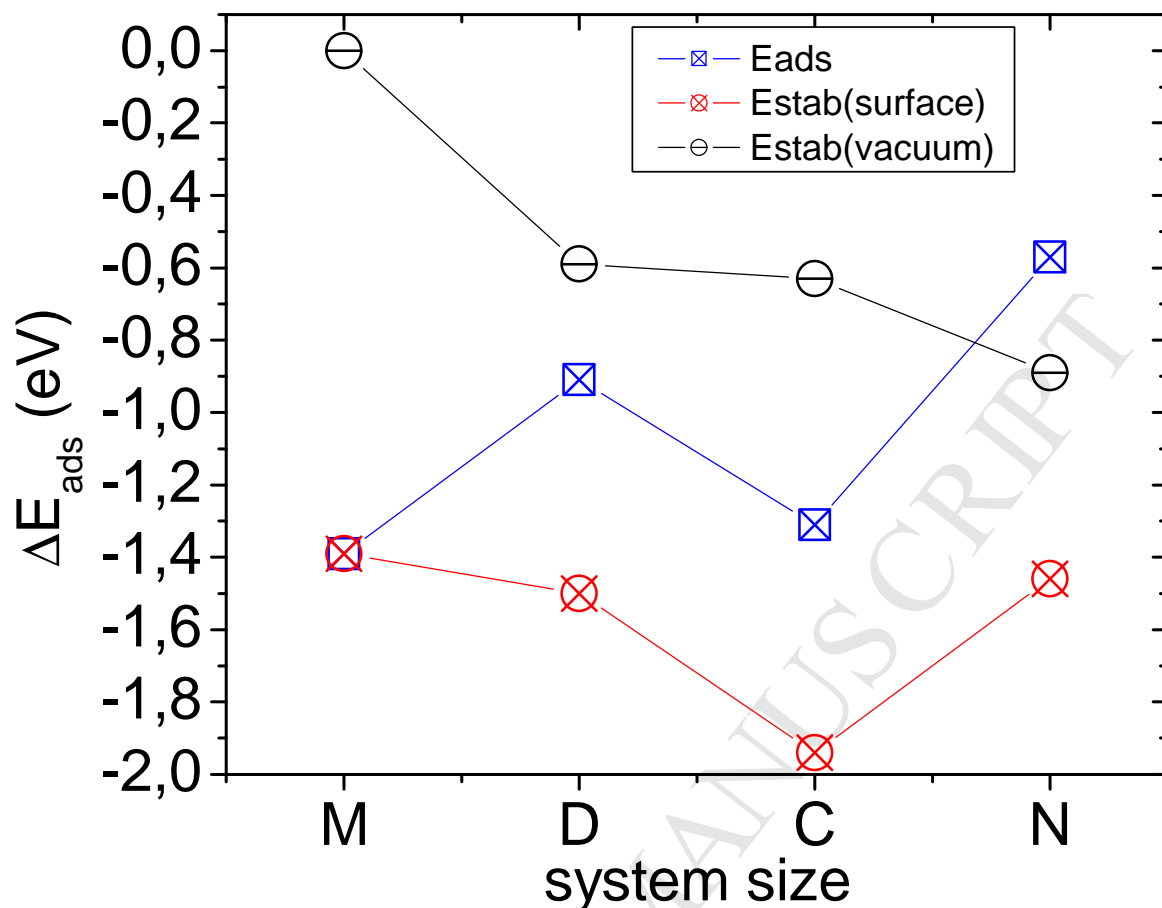
Figure 3: Stabilization and adsorption energies variation as a function of the melamine cluster size. M, D, C, N stand respectively for Monomer, Dimer, Chain and Network of melamine.
