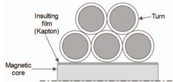
Fig. 7. Structure with an insulated core.
