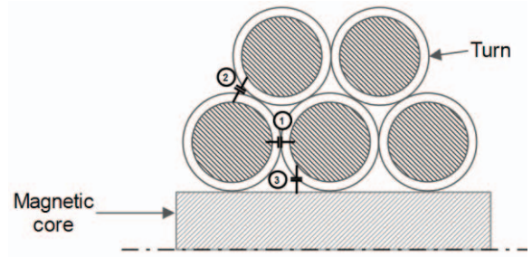
Fig. 3. Representation of capacitive couplings between turns and core.
