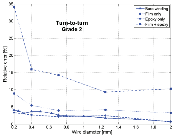
Fig. 15. Comparison of results for turn-to-turn capacitance for Grade 2.
