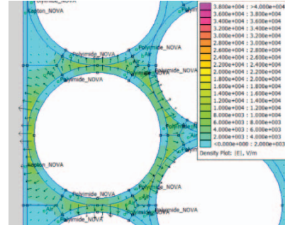
Fig. 13. Segmentation and field lines contained in the specified regions for energy calculation.
