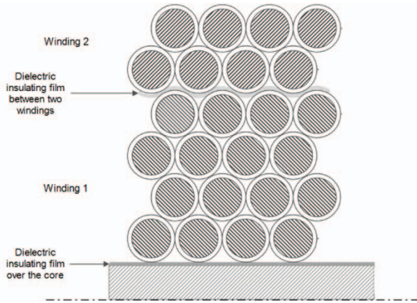
Fig. 2. Cross-sectional view of a portion of concentrated winding.
