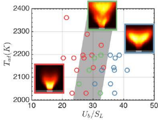
FIGURE 6. Position of the leading reaction edge of N_2 -diluted CH_4 /air lean flames at S_0 = 0.75 as a function of T_{ad} and U_b/S_L . The flame leading edge is located inside z_f/r_0 < 0 (red) or outside z_f/r_0 > 0 (blue) the injector. Green symbols indicate undetermined states with oscillations between these two states. The grey zone roughly delineates the transition region where it is difficult to safely determine the leading edge flame position.
