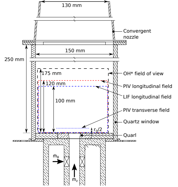
FIGURE 1. OXYTEC atmospheric test-rig.
