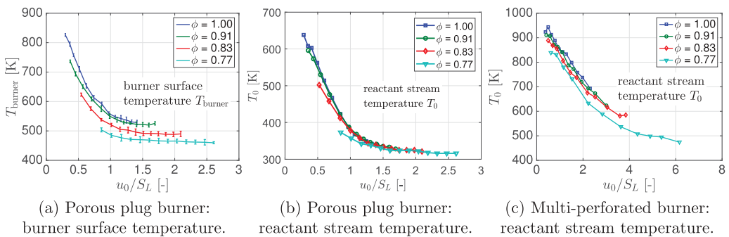
Figure 6. Burner and reactant stream temperature measurements as a function of u_0/S_L . u_0 : gas flow velocity at the burner outlet. S_L : adiabatic laminar burning velocity at T_0 .
