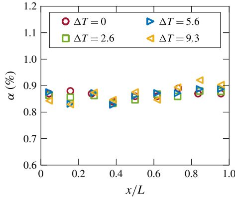
FIGURE 7. (Colour online) The profile of the gas volume fraction for \alpha = 0.9\% at half-height for different imposed temperature differences between hot and cold wall \Delta T .
