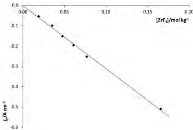
Fig. 3. Linear relationship between the cathodic peak current density and the \text{ZrF}_4 content in the bath in the LiF NaF system on Ag electrode at 100 \text{ mV s}^{-1} and 750^\circ\text{C} .
