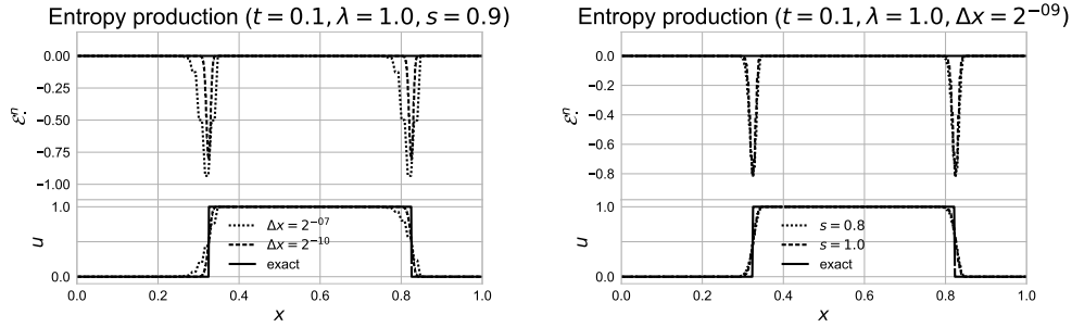
Fig. 5. Local in space numerical entropy production of the advection equation with initial condition ( I_B ) for varying space steps \Delta x at left and for varying relation parameters s at right. The numerical and exact solutions at t = 0.1 are shown below and the corresponding entropy productions above.
