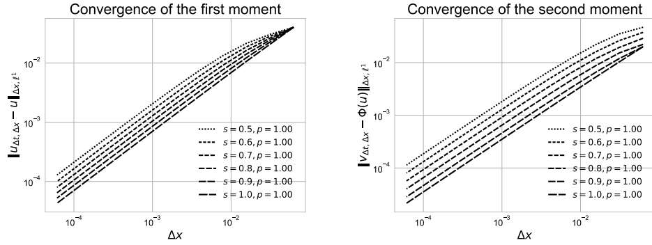
Fig. 2. Initial condition ( I_A ). Error in norm \ell^1 of the numerical solution of the advection equation (30) according to the space steps \Delta x for several relaxation parameter values s \in \{0.5, 0.6, 0.7, 0.8, 0.9, 1.0\} . p is the convergence rate.
