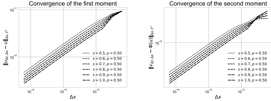
Fig. 3. Initial condition ( I_B ). Error in norm \ell^1 of the numerical solution of the advection equation (30) according to the space steps \Delta x for several relaxation parameter values s \in \{0.5, 0.6, 0.7, 0.8, 0.9, 1.0\} . p is the convergence rate.
