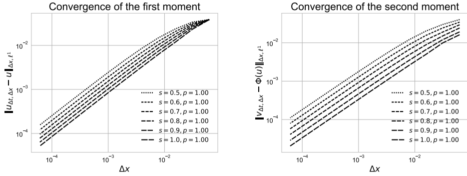
Fig. 6. Initial condition ( I_A ). Error in norm \ell^1 of the numerical solution of the Burgers equation (31) according to the space steps \Delta x for several relaxation parameter values s \in \{0.5, 0.6, 0.7, 0.8, 0.9, 1.0\} . p is the convergence rate.
