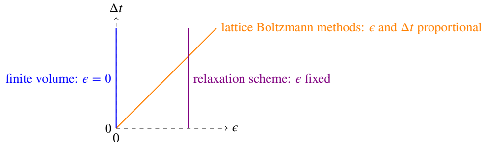
Fig. 1. Representation of the schemes parameters in the plane (\epsilon, \Delta t) .
