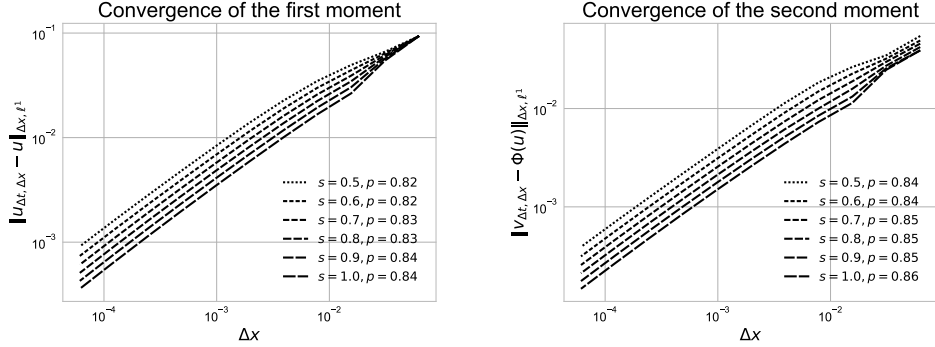
Fig. 7. Initial condition ( I_B ). Error in norm \ell^1 of the numerical solution of the Burgers equation (31) according to the space steps \Delta x for several relaxation parameter values s \in \{0.5, 0.6, 0.7, 0.8, 0.9, 1.0\} . p is the convergence rate.
