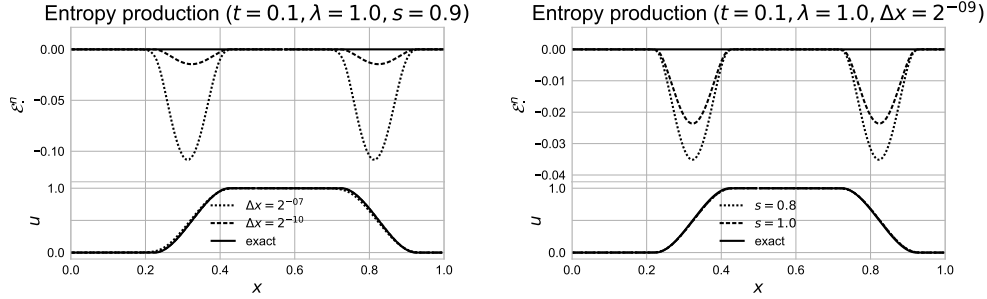
Fig. 4. Local in space numerical entropy production of the advection equation with initial condition ( I_A ) for varying space steps \Delta x at left and for varying relation parameters s at right. The numerical and exact solutions at t = 0.1 are shown below and the corresponding entropy productions above.
