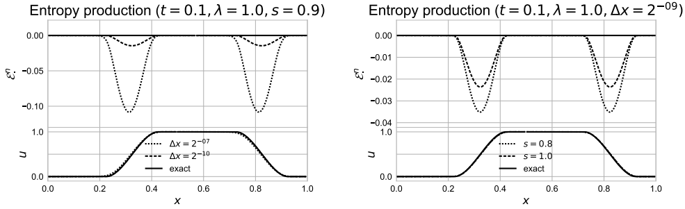
Fig. 2. Local in space numerical entropy production of the advection equation with initial condition (I_A) for varying space steps \Delta x at left and for varying relation parameters s at right. The numerical and exact solutions at t = 0.1 are shown below and the corresponding entropy productions above.
