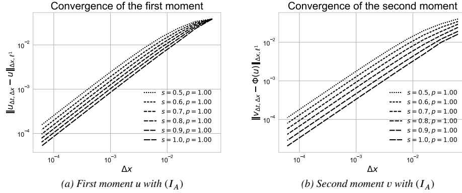
Fig. 4. Error in norm \ell^1 of the numerical solution of the Burgers equation (33) according to the space steps \Delta x for several relaxation parameter values s \in \{0.5, 0.6, 0.7, 0.8, 0.9, 1.0\} . p is the convergence rate.
