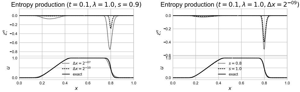
Fig. 5. Local in space numerical entropy production of the Burgers equation with initial condition (I_A) for varying space steps \Delta x at left and for varying relation parameters s at right. The numerical and exact solutions at t = 0.1 are shown below and the corresponding entropy productions above.
