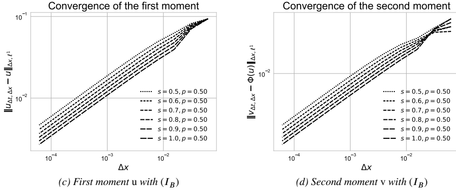
Fig. 1. Error in norm \ell^1 of the numerical solution of the advection equation (32) according to the space steps \Delta x for several relaxation parameter values s \in \{0.5, 0.6, 0.7, 0.8, 0.9, 1.0\} . p is the convergence rate.
