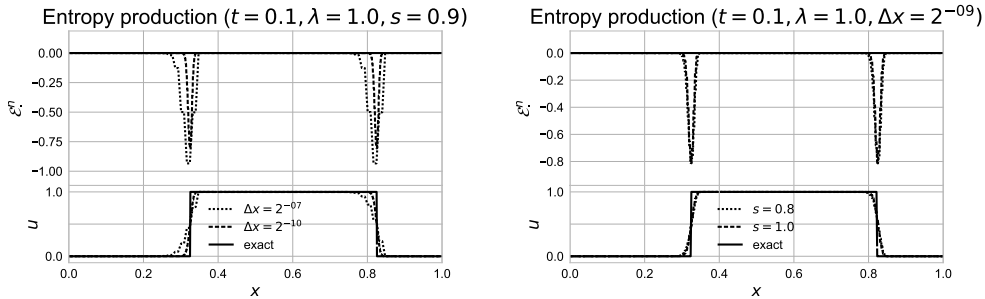
Fig. 3. Local in space numerical entropy production of the advection equation with initial condition (I_B) for varying space steps \Delta x at left and for varying relation parameters s at right. The numerical and exact solutions at t = 0.1 are shown below and the corresponding entropy productions above.
