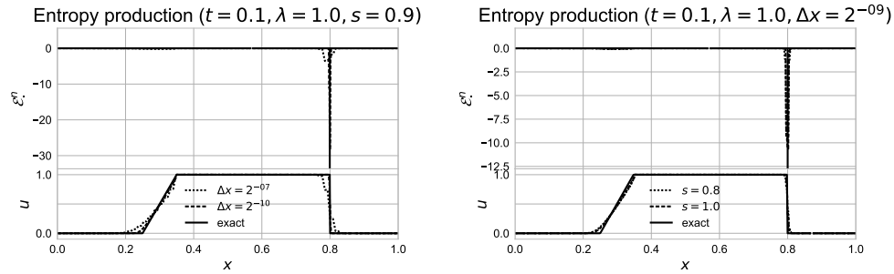
Fig. 6. Local in space numerical entropy production of the Burgers equation with initial condition (I_B) for varying space steps \Delta x at left and for varying relation parameters s at right. The numerical and exact solutions at t = 0.1 are shown below and the corresponding entropy productions above.
