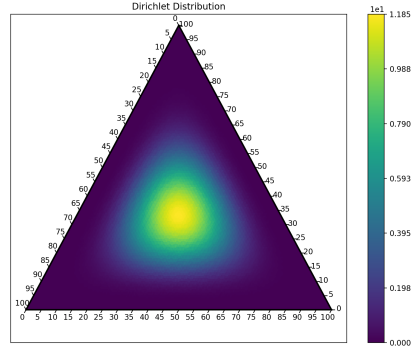
Figure 3: Ternary Density plot of a \text{Dir}(5, 5, 5) . We observe a mode at \left(\frac{1}{3}, \frac{1}{3}, \frac{1}{3}\right) .
