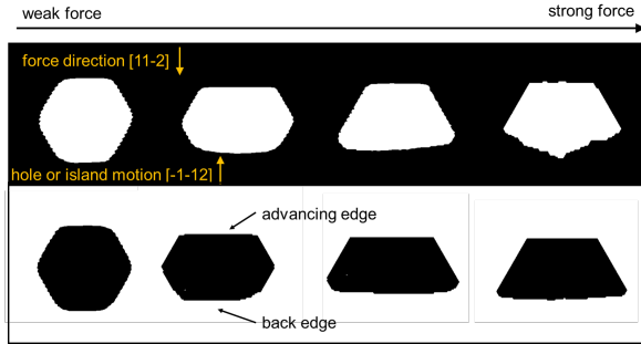
Figure 5: Shapes of a 2D island (first line) and a 2D hole (second line) on a (111) surface under a force that adds a bias to diffusion. The force is towards the bottom of the image. The force acting on the shapes implies an energy change from left to right E_{cg} = 0.0001, 0.001, 0.01, 0.1 E_b .
