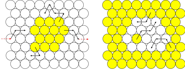
Figure 1: (111) surface pattern. Yellow circles represent occupied positions (top layer), while white circles are empty positions. The figure on the left represents a 2D one-atom-thick island, while that on the right shows a 2D vacancy island with an adatom in the middle. Some possible trajectories of atoms are shown with arrows. The red arrows give an idea of the boundary conditions for a jump at the edges of the simulation box.
