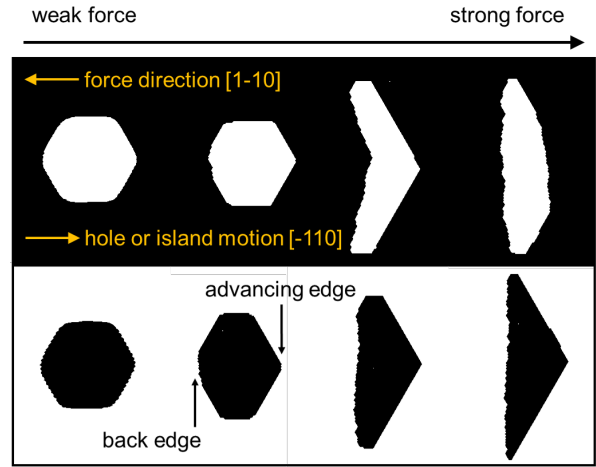
Figure 4: Shapes of a 2D island (white, first line) and a 2D hole (black, second line) on a (111) surface under a force that adds a bias to diffusion. The force is towards the left of the image. The force acting on the shapes on the right is higher than that acting on the shapes on the left. From left to right E_{cg} = 0.0001, 0.001, 0.01, 0.1 E_b . k_B T = 0.1 E_b .
