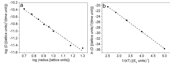
Figure 2: a: log-log plot of the diffusion coefficient of islands (with- out force) as a function of the radius at k_B T = 0.3 E_b . b: diffusion coefficient of an island with radius=10 lattice units (without force) as a function of temperature.
