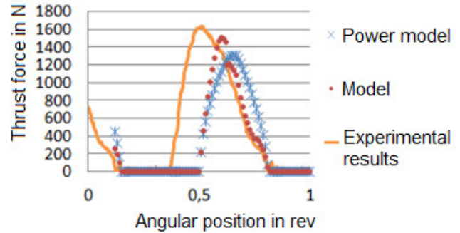
Fig. 10. Comparison of experimental and theoretical thrust forces for f = 0.2 \text{ mm}\cdot\text{rev}^{-1} and a = 0.5 \text{ mm} .
