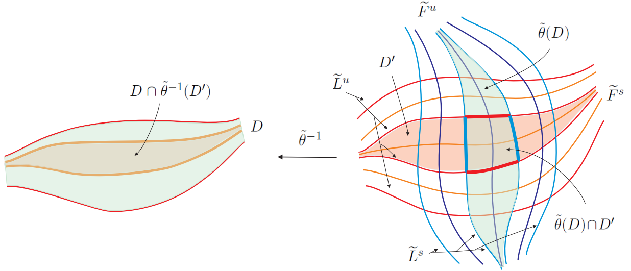
Figure 3: The proof of Proposition 2.12
