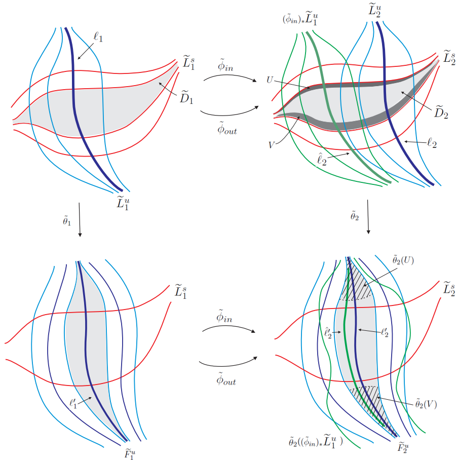
Figure 4: Proof of Lemma 3.10
