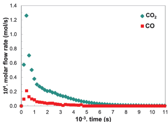
Fig. 3 . Molar flow rates of CO_2 and CO during the combustion at 643 K under air.
