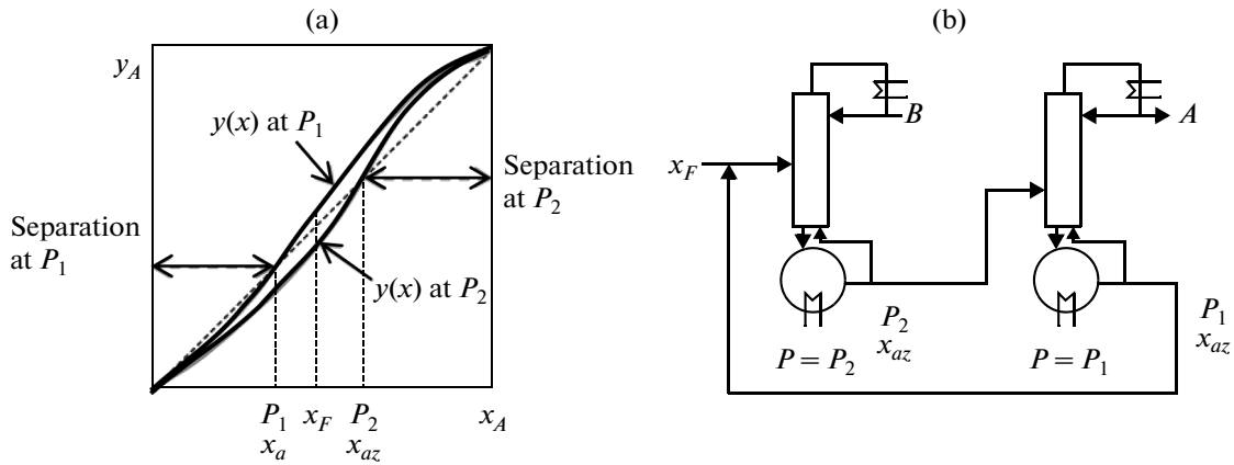
Fig. 7. (a) Effect of pressure on the azeotropic composition and (b) corresponding continuous pressure-swing distillation process.
