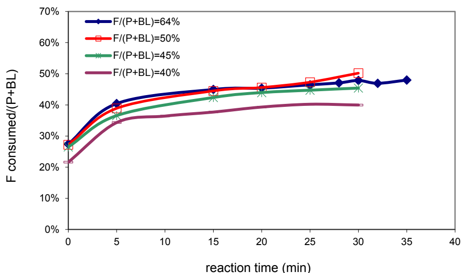
Fig. 6. Formaldehyde consumption during 50-BPF synthesis with varied formaldehyde initial ratio
