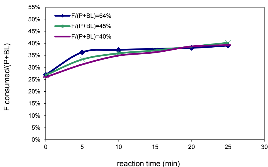
Fig. 7. Formaldehyde consumption during 60-BPF synthesis with varied formaldehyde initial ratio
