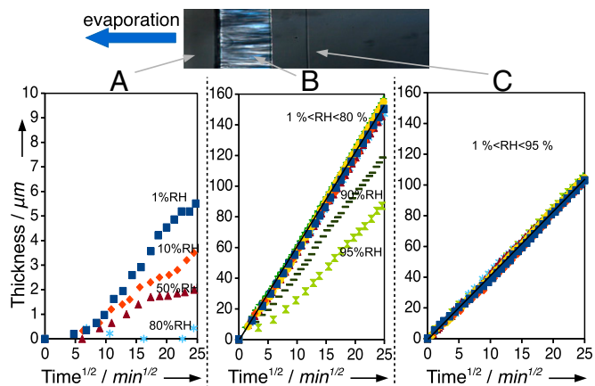
Fig. 4. The increase in thickness of different phases in the interfacial layer as a function of time, as obtained from the optical microscopy images (Top) (DDM/water system). The air RH varies between 0% and 95%. (A) The thickness of the external lamellar phase in contact with air depends on RH, and this phase disappears for \text{RH} > 85\% . (B) The thickness of the hexagonal phase is independent of RH until the disappearance of the outer lamellar phase at \text{RH} > 85\% . (C) The thickness of the micellar cubic phase is always independent of RH.
