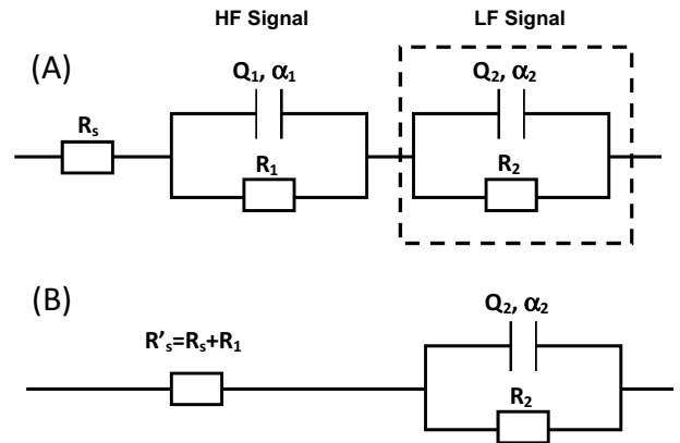
Fig. 4. (A) R_s + Q_1 // R_1 + Q_2 // R_2 model to fit two distinct depressed semi-circles observed on Nyquist plot. R_s = solution resistance, R_1 and R_2 resistances corresponding to the circle diameters at HF and LF respectively, Q_1 , \alpha_1 and Q_2 , \alpha_2 the characteristic parameters of constant phase elements at HF and LF respectively. (B) R'_s + Q_2 // R_2 model to fit the depressed semi-circle observed at LF taking only the LF contribution into account. R'_s = R_s + R_1 .
