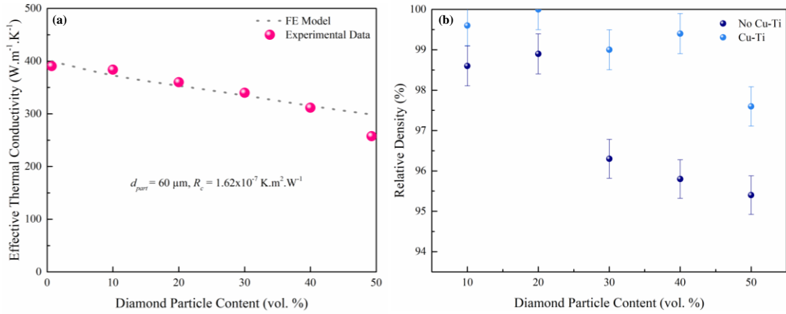
Figure 6: (a) Measured (pink spheres) and calculated (dashed line) thermal conductivities of Cu/D composite materials reinforced with diamond particles of d_{part} = 60 \mu\text{m} and an interfacial thermal resistance of (1.62 \pm 0.15) \times 10^{-7} \text{ K.m}^2.\text{W}^{-1} . (b) Relative density of composite materials with respect to the diamond volume fraction with and without Cu-Ti addition.
