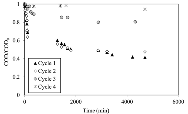
Fig. 5. Carbon oxygen demand (COD) removal during 4 cycles, [TiO 2 ] = 0.4 g/L.
