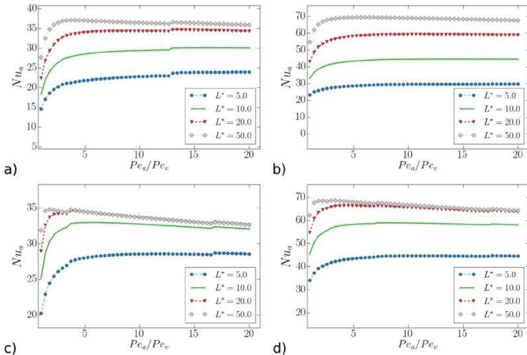
Fig. 9. Arterial Nusselt Nu_a versus Péclet ratio Pe_a/Pe_v for several vessels length L^* 5,10,20,50, and several venous Péclet and distance between vessels: (a) Pe_v 5, \alpha 0.2, (b) Pe_v 10, \alpha 0.2, (c) Pe_v 5, \alpha 0.5, (d) Pe_v 10, \alpha 0.5.
