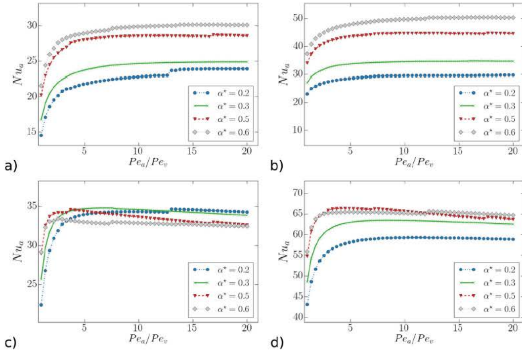
Fig. 8. Arterial Nusselt Nu_a versus Péclet ratio Pe_a/Pe_v for several distances between vessels \alpha^* 0.2,0.3,0.5,0.6 and several venous Péclet Pe_v and vessels length L^* : (a) Pe_v 5, L^* 5, (b) Pe_v 10, L^* 5, (c) Pe_v 5, L^* 20, (d) Pe_v 10, L^* 20.
