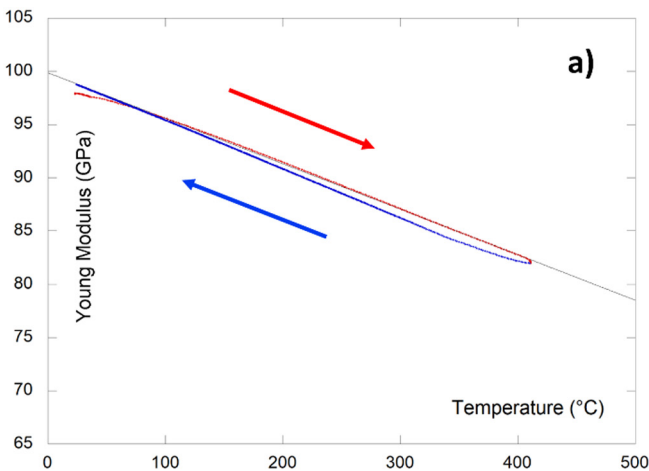
Fig. 3. Vibration measurement of Young modulus during heating and cooling cycle up to a) 400^\circ C and b) 700^\circ C.
