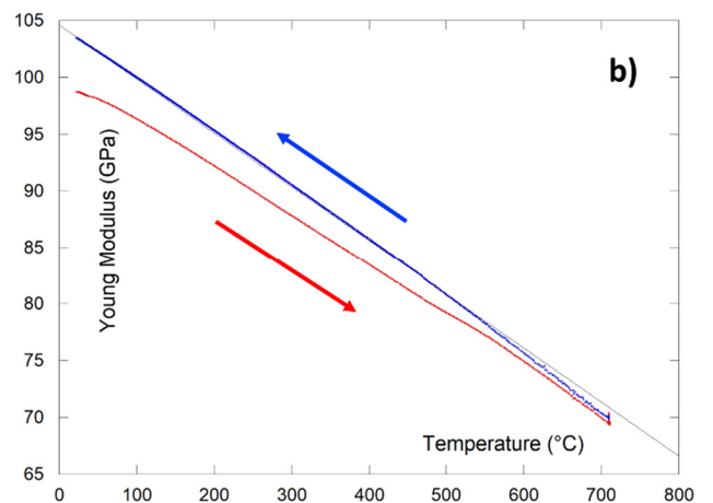
Fig. 3. Vibration measurement of Young modulus during heating and cooling cycle up to a) 400^\circ C and b) 700^\circ C.
