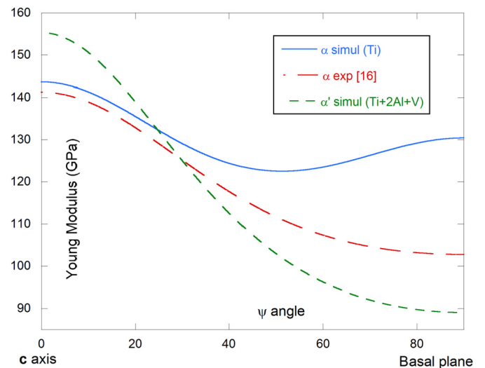
Fig. 4. Young modulus along a direction inclined by the angle \psi with respect to the c axis of the hexagonal structure.
