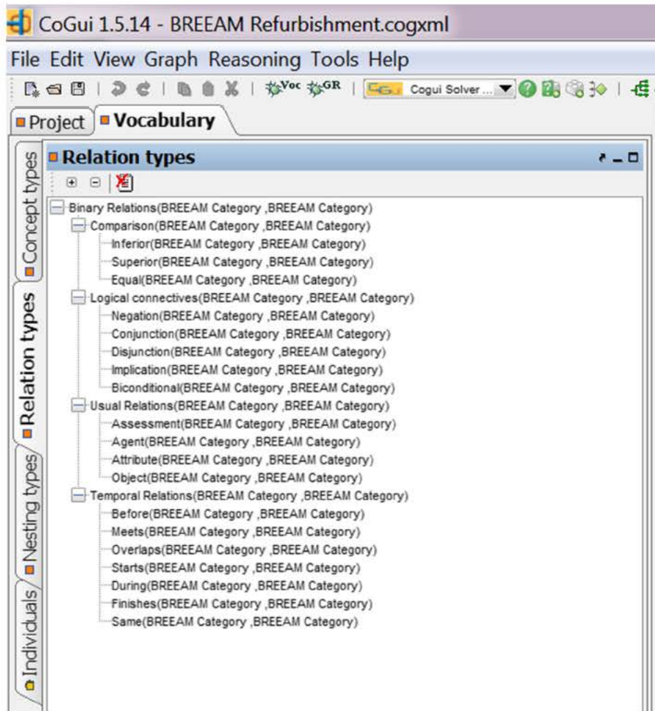
Fig. 5. Relation types in a subPropertyOf hierarchy.
