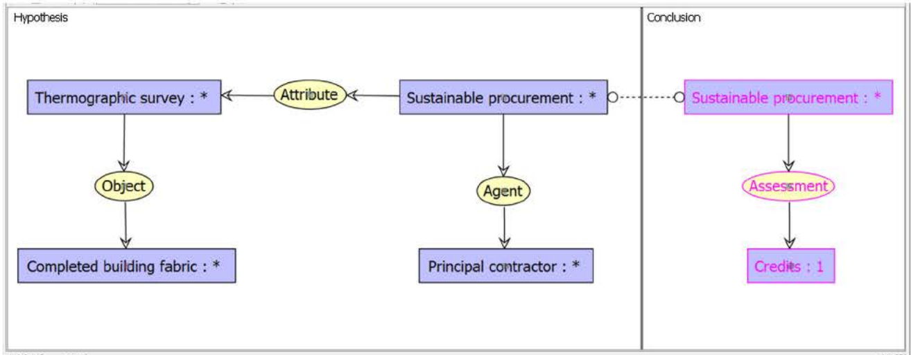
Fig. 7. A rule modelling a sustainable procurement assessment.
