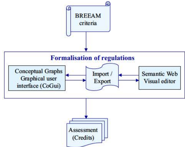
Fig. 3. Implementation process into CoGui.
