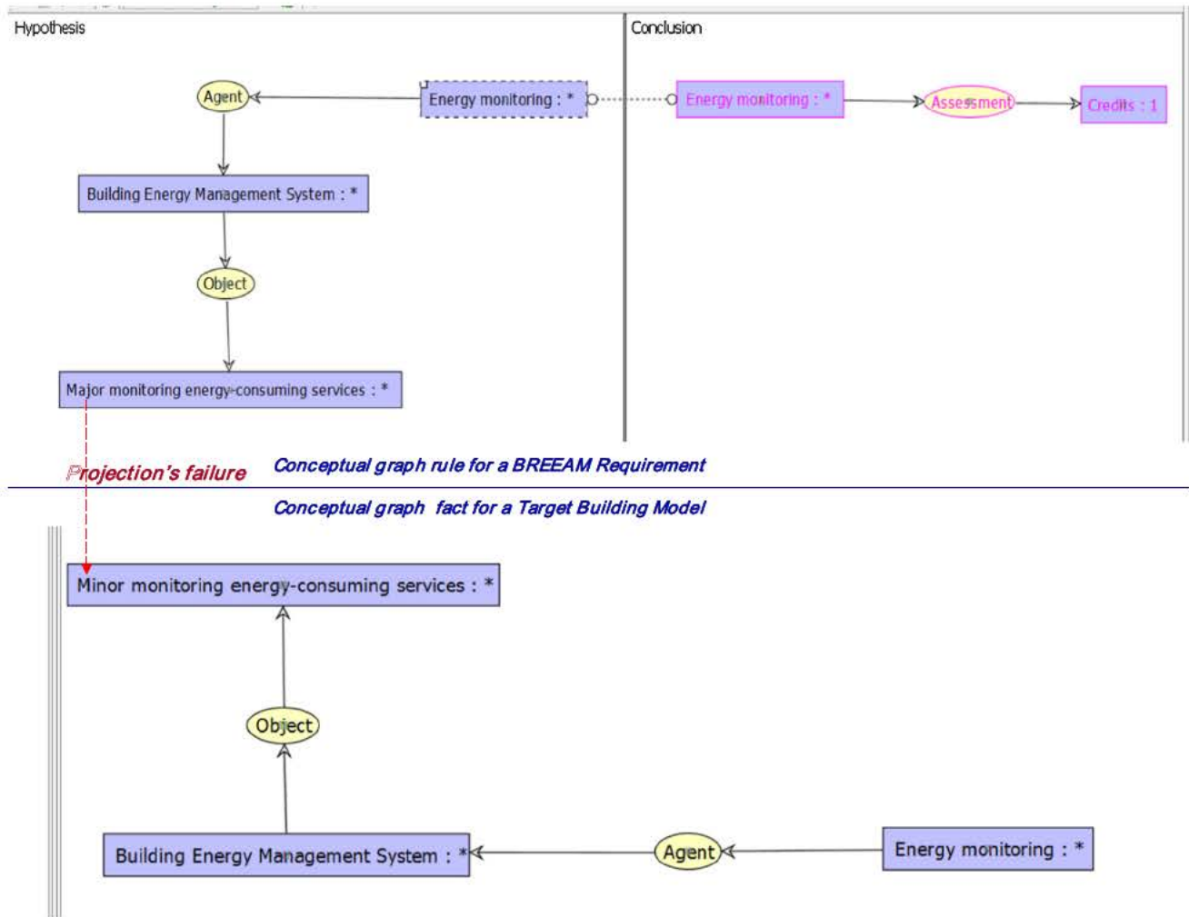
Fig. 10. A compliance checking with the rule of energy monitoring.
