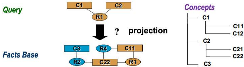
Fig. 6. Projection operation for information retrieval.
