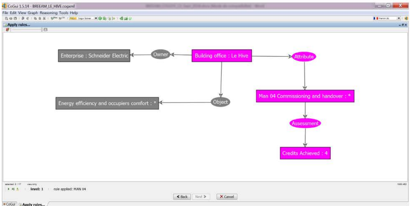
Fig. 13. Conceptual graph rule application for BREEAM Rating of the “Le HIVE”.
