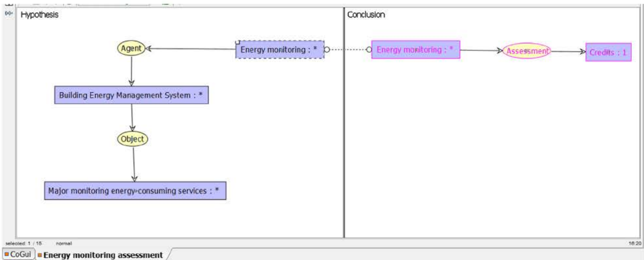
Fig. 9. A rule modelling an Energy monitoring assessment.
