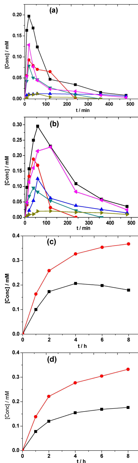
Figure 7. Evolution of concentration of formed (a, b) carboxylic acid: (■) oxalic, (●) Maleic, (▲) oxamic, (▼) malic, (◄) glyoxylic and (►) acetic acids; and (c, d) inorganic ions: (●) \text{NH}_4^+ and (■) \text{NO}_3^- vs electrolysis time during the EF ( 0.2 \text{ mM Fe}^{2+} ) treatment of 0.192 \text{ mM} ( 30 \text{ mg L}^{-1} TOC) 4-APZ in 0.05 \text{ M Na}_2\text{SO}_4 solution using (a,c) BDD and (b,d) \text{Ti}_4\text{O}_7 anodes at 120 mA and pH 3.
