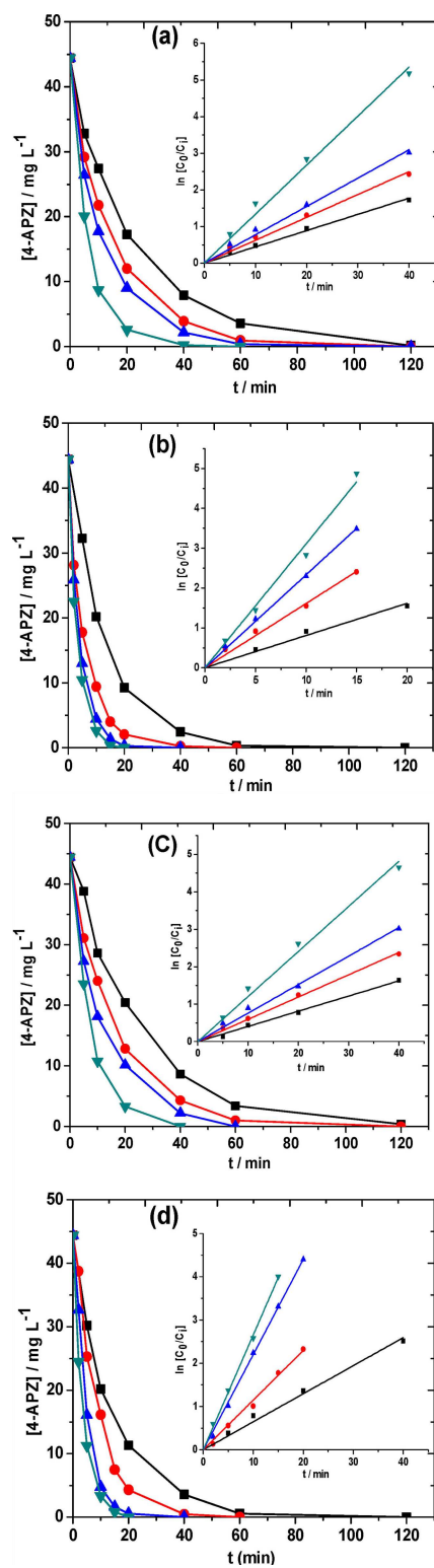
Figure 1. Decay of 4-APZ concentration vs electrolysis time for the (a, c) AO-H 2 O 2 and (b, d) EF (0.2 mM Fe 2+ ) treatments of 0.192 mM (44.4 mg L -1 ) 4-APZ in 0.05 M Na 2 SO 4 solutions at applied current of (■) 30 mA, (●) 60 mA, (▲) 120 mA and (▼) 250 mA using (a, b) BDD and (c, d) Ti 4 O 7 anodes. The corresponding kinetic analyses assuming the oxidation of 4-APZ by • OH follows pseudo-first order kinetic are given in the inset panels.
