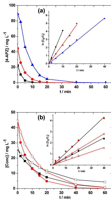
Figure 2. (a) Decay of 4-APZ concentration vs electrolysis time for the EF (0.2 mM Fe 2+ ) treatment of (■) 0.096 mM, (●) 0.192 mM and (▲) 0.384 mM 4-APZ in 0.05 M Na 2 SO 4 solution at applied current of 120 mA using BDD anode and (b) Decay of concentration of (●, ○) 4-APZ and (■, □) pHBA vs electrolysis time during EF treatment of the solutions containing 0.192 mM of each compound at applied current of (○, □) 60 mA and (●, ■) 120 mA using BDD anode. The corresponding kinetic analyses assuming the oxidation of 4-APZ and/or pHBA by • OH following pseudo-first order kinetic are given in the inset panels.
