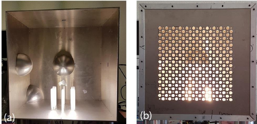
Fig. 1: Photography of the cavity without (a) and with (b) the front face made of drilled holes. The FLs inside can be separately excited using an Arduino.
