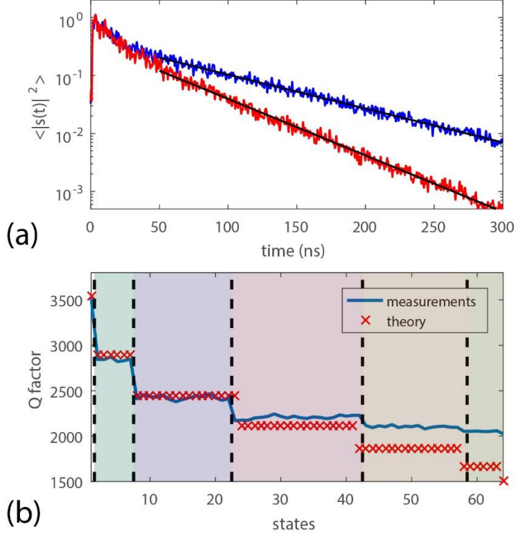
Fig. 3: (a) Plot of the transmitted intensity in time-domain averaged over the near-field of the aperture for 1 (blue line) and 3 (red line) FLS that are turned on. The black lines are exponential fits, \langle I(t) \rangle = e^{-\frac{t}{\tau}} . (b) Q factor found from reverberation times \tau as a function of the state. The number of FLS that are turned on is indicated by upper horizontal numbers.
