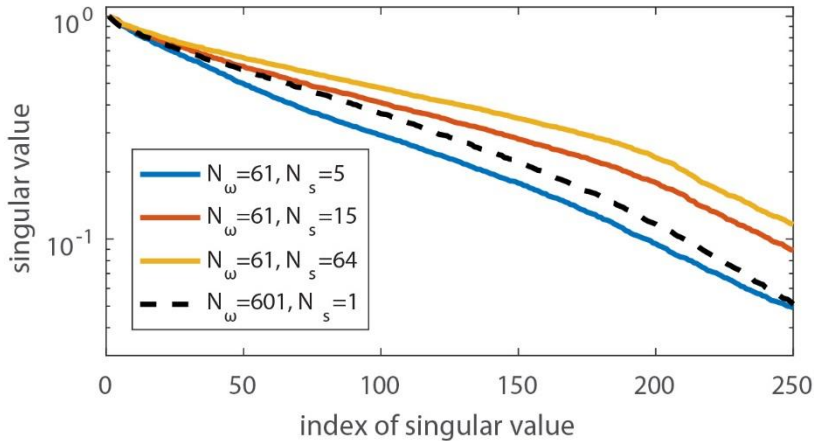
Fig. 5: Variation of the normalized singular values of the sensing matrix of the cavity with their index for different number of states N_s taken into account and N_\omega = 61 frequencies chosen randomly within the bandwidth. These variations are compared to the “unloaded” case N_s = 1 for which all the FLs are switched off but the entire frequency range is used, N_\omega = 601 .
