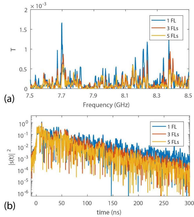
Fig. 2: (a) Spectra of transmission coefficients between the first port of the cavity and a point in the near-field of the cavity for three different states corresponding to one, three and five FLs that are turned on. (b) Transmitted intensity in time-domain for these three different states.
