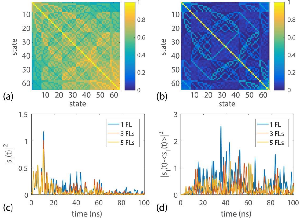
Fig. 4: (a,b) Covariance matrix as a function of the state number averaged over the frequency range for (a) near-field scan and (b) the differential approach (the field averaged over the states is subtracted). (c,d) Plot of the transmitted intensity in the time domain for (c) the near-field scan and (d) the differential approach. The averaging of \langle s_i(t) \rangle_i is performed on the 64 states of the cavity.
