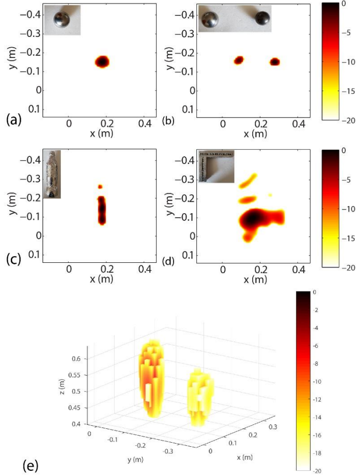
Fig. 6: (a) Reconstructed images of 4 objects at a distance of 52 cm from the aperture of the leaky cavity with N_f=61 and N_s=12 : a single (a) and two spheres (b) of 5-cm diameter; (c) a metallic bottle of height 25 cm and diameter 9 cm; and (d) a metallic L-shaped phantom. (e) 3D reconstruction of the two spheres shown in (b).
