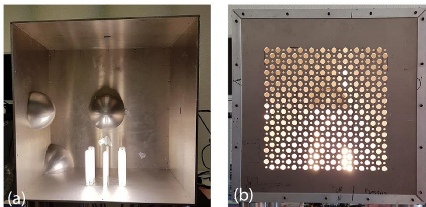
Fig. 1: Photography of the cavity without (a) and with (b) the front face made of drilled holes. The FLs inside can be separately excited using an Arduino.
