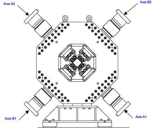
Fig. 3 Visualization of the biaxial testing machine
