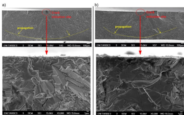
Fig. 8 SEM observations of crack propagation and cracked carbides on rupture facies of cruciform specimens under in-plane biaxial cyclic loading. a) proportional equibiaxial tension-tension test at 95 kN; b) proportional tension-tension test at 60 kN / 89 kN
